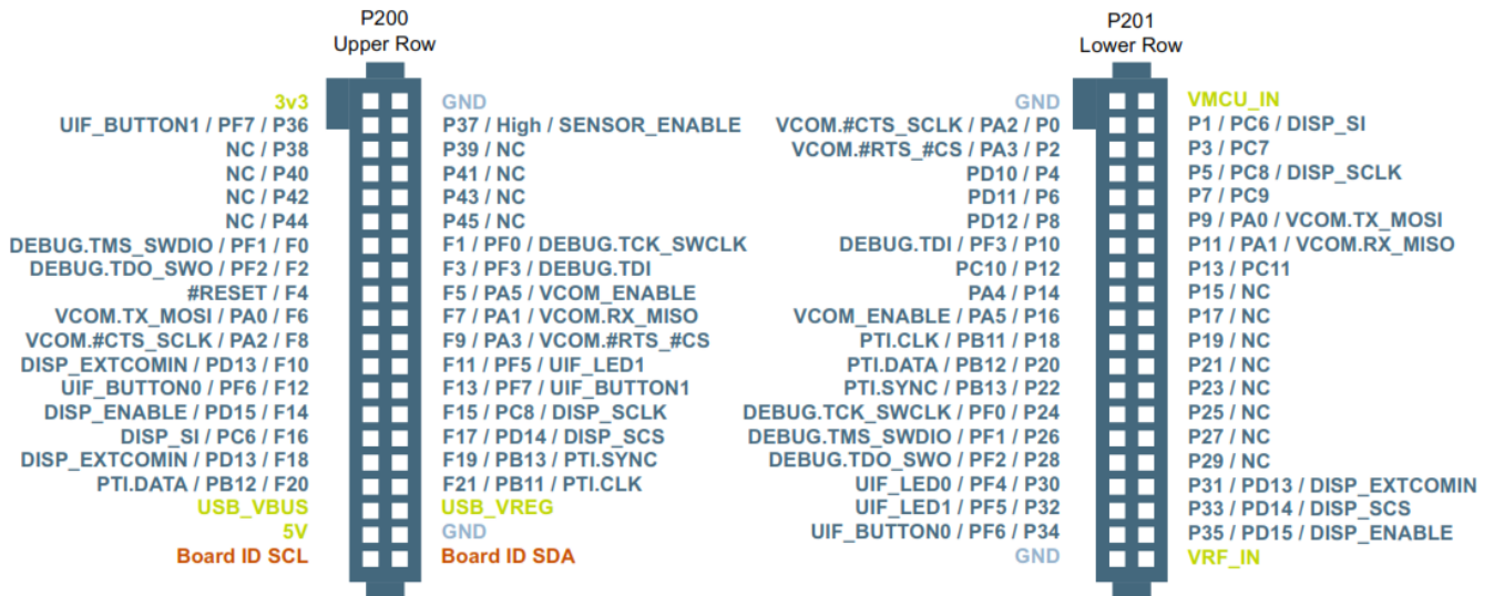
Figure 2.1. BRD4100A Radio Board Connector Pin Mapping
