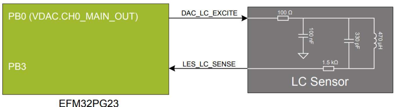
Figure 6.4. LC Metal Sensor
