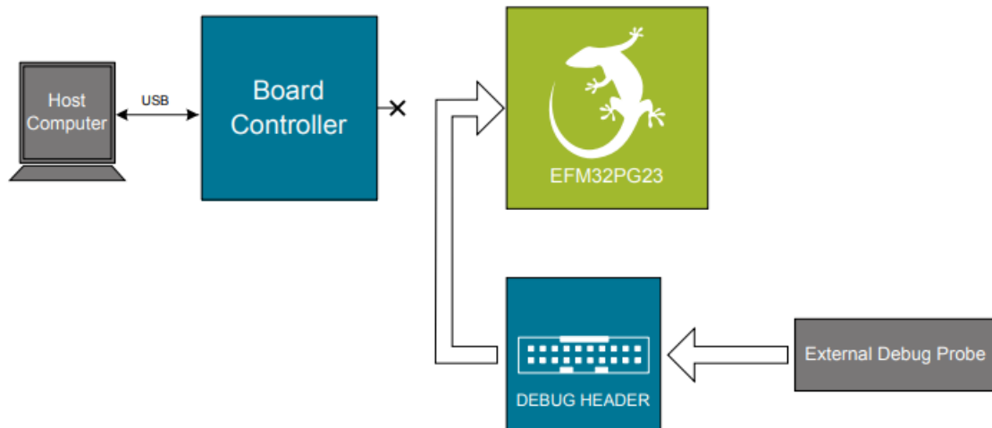
Figure 8.3. Debug IN
