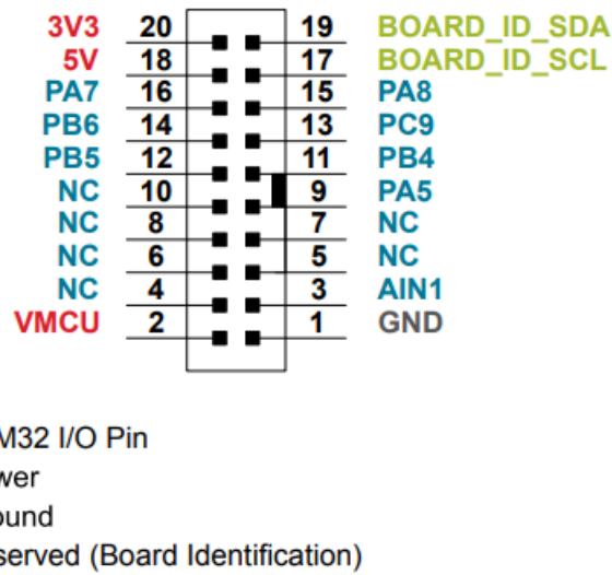
Figure 4.2. EXP Header
