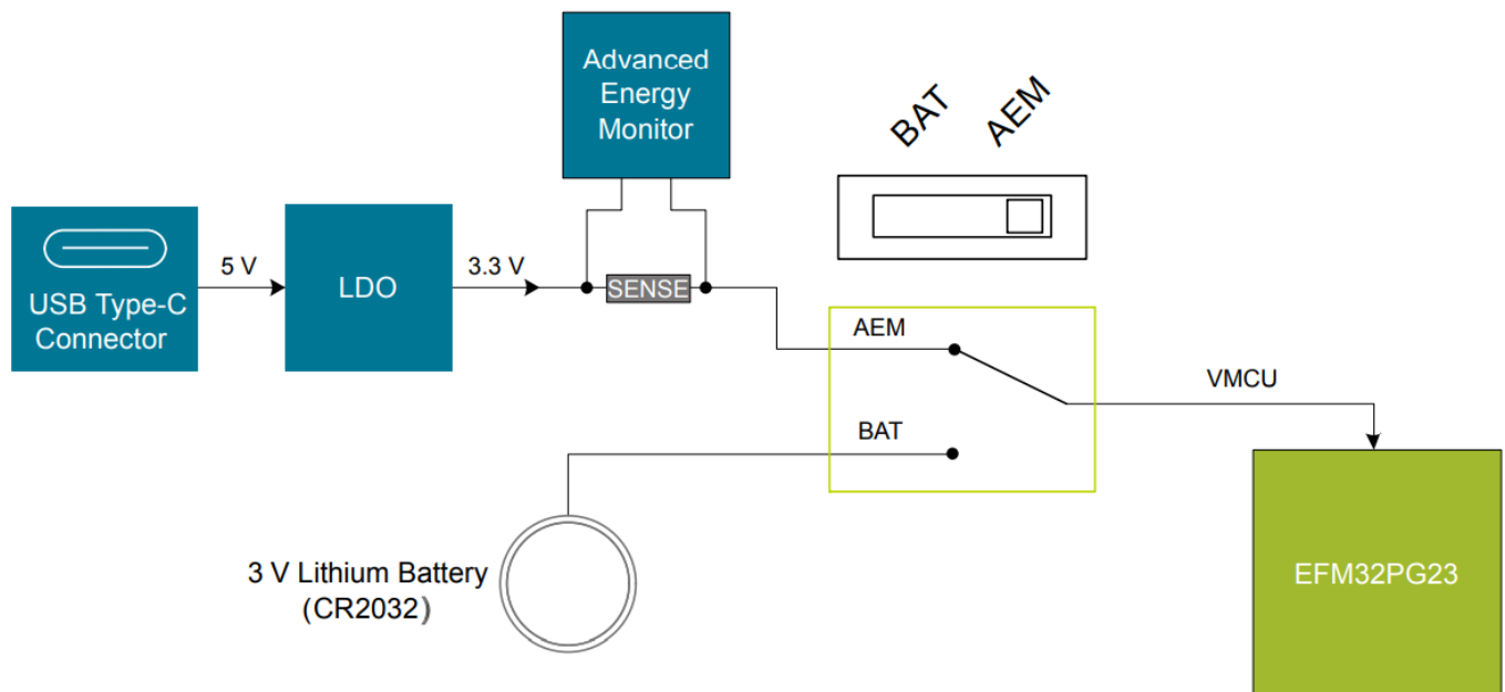
Figure 5.1. Power Switch
