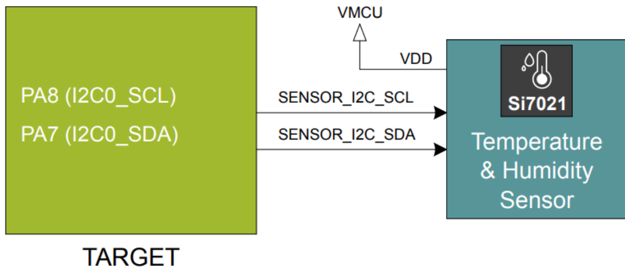
Figure 6.3. Si7021 Relative Humidity and Temperature Sensor
