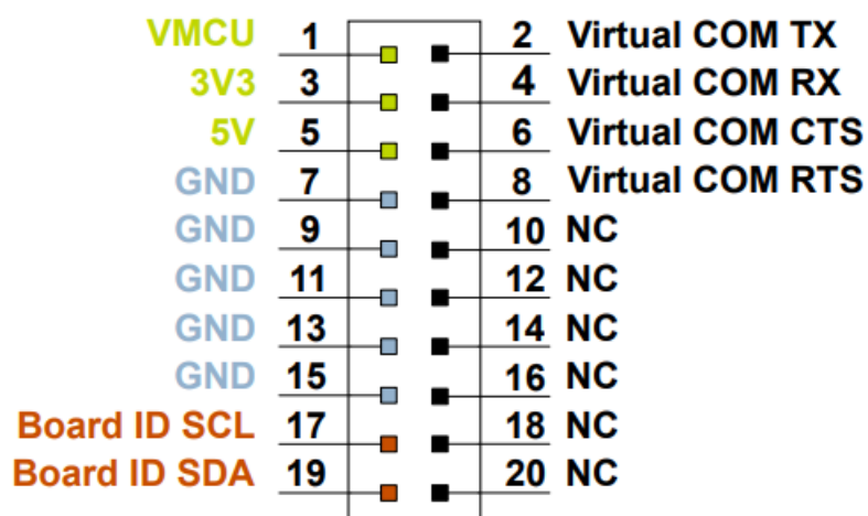
Figure 4.4. Simplicity Connector
