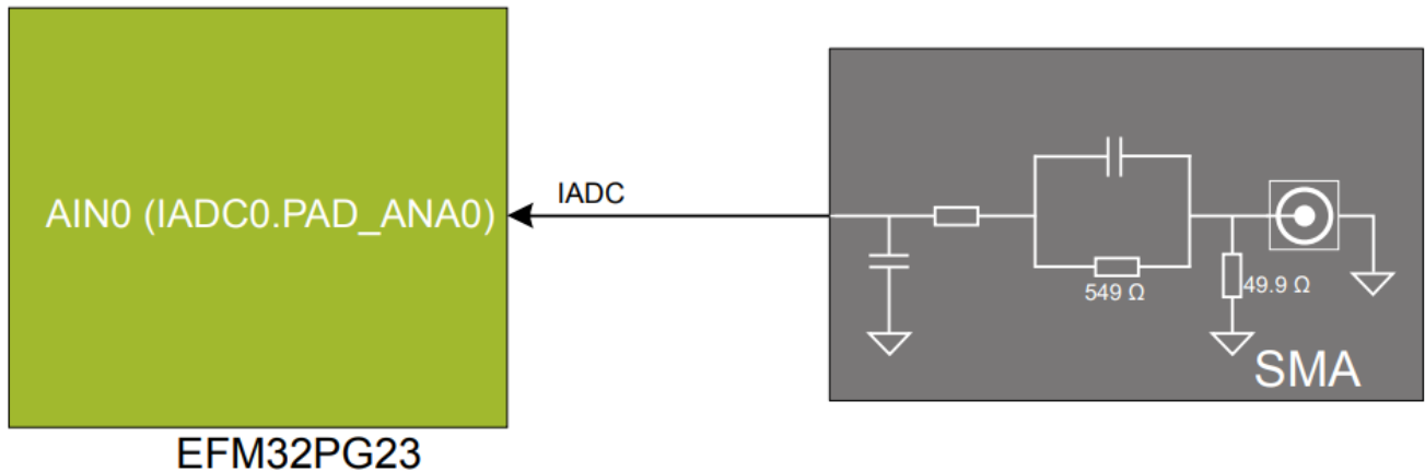
Figure 6.5. SMA Connector
