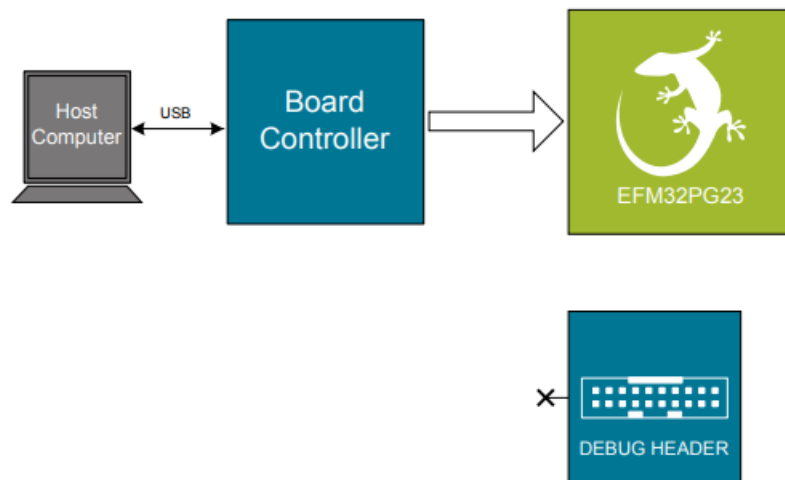
Figure 8.1. Debug MCU
