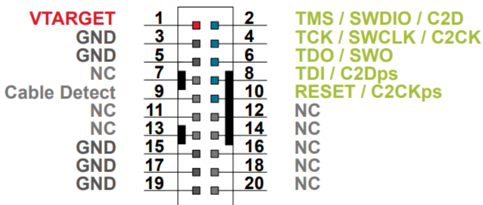
Figure 4.3. Debug Connector
