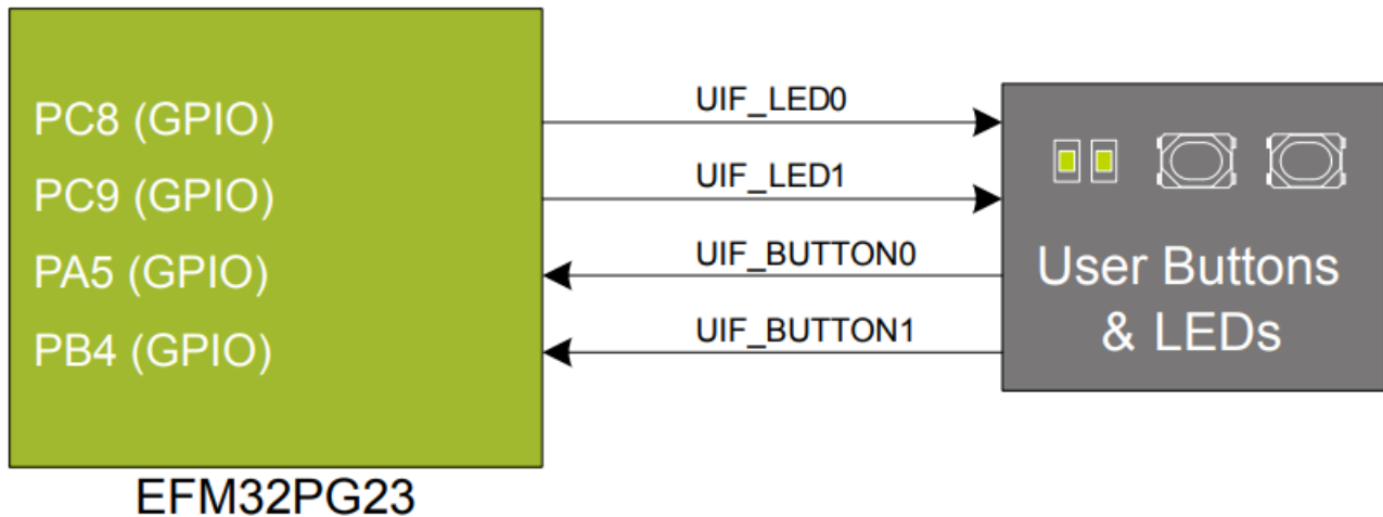
Figure 6.1. Buttons and LEDs
