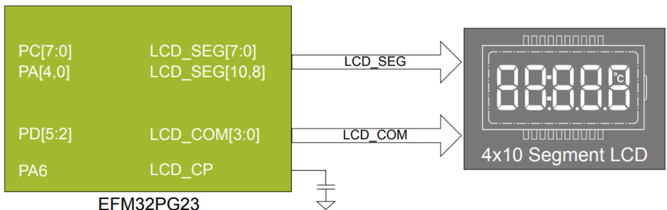
Figure 6.2. Segment LCD
