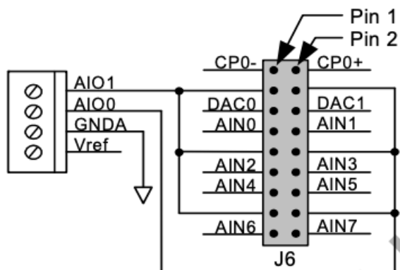
Figure 3. J6 Analog I/O Configuration Connector
