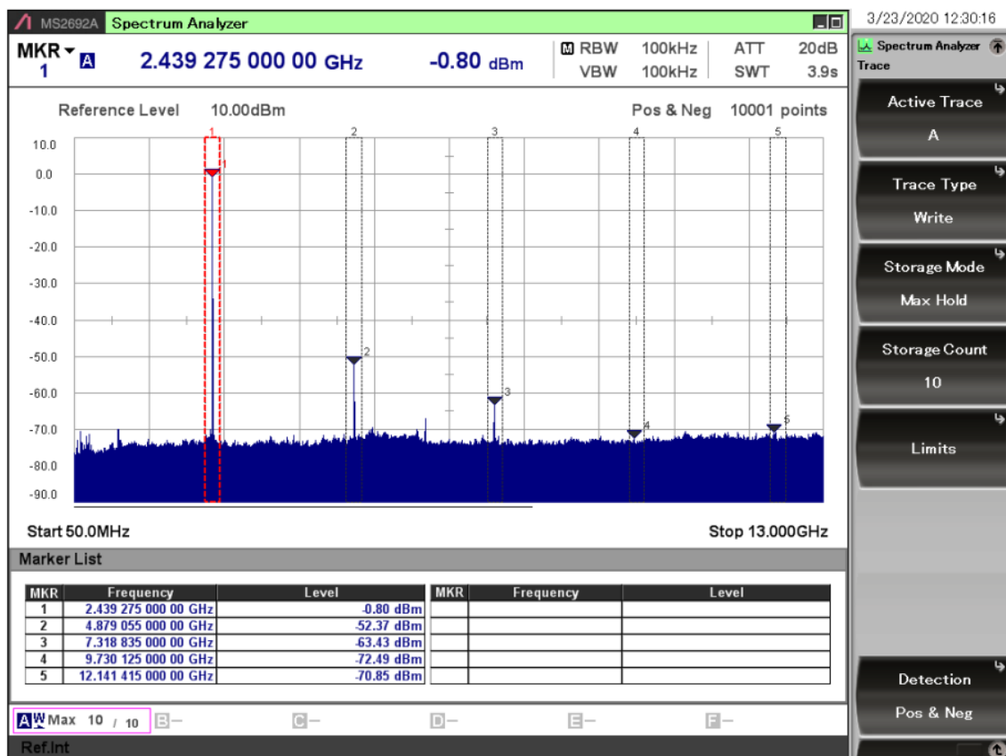
Figure 6.1. Typical Output Spectrum of the BRD4310A; PAVDD = 3.3 V
