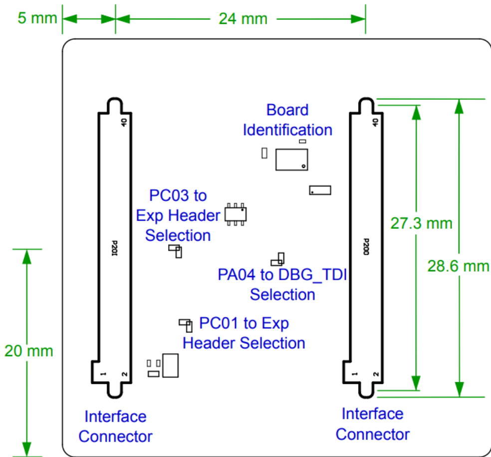
Figure 4.2. BRD4310A Bottom View
