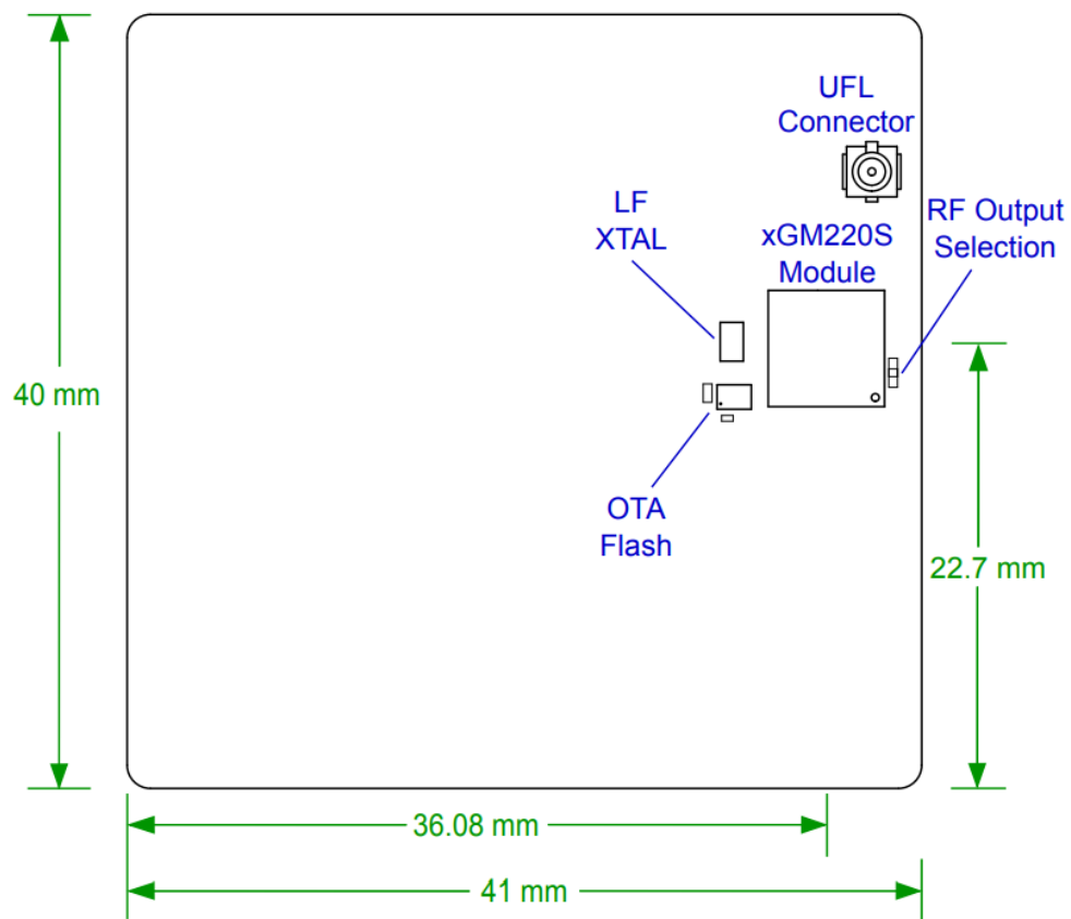
Figure 4.1. BRD4310A Top View
