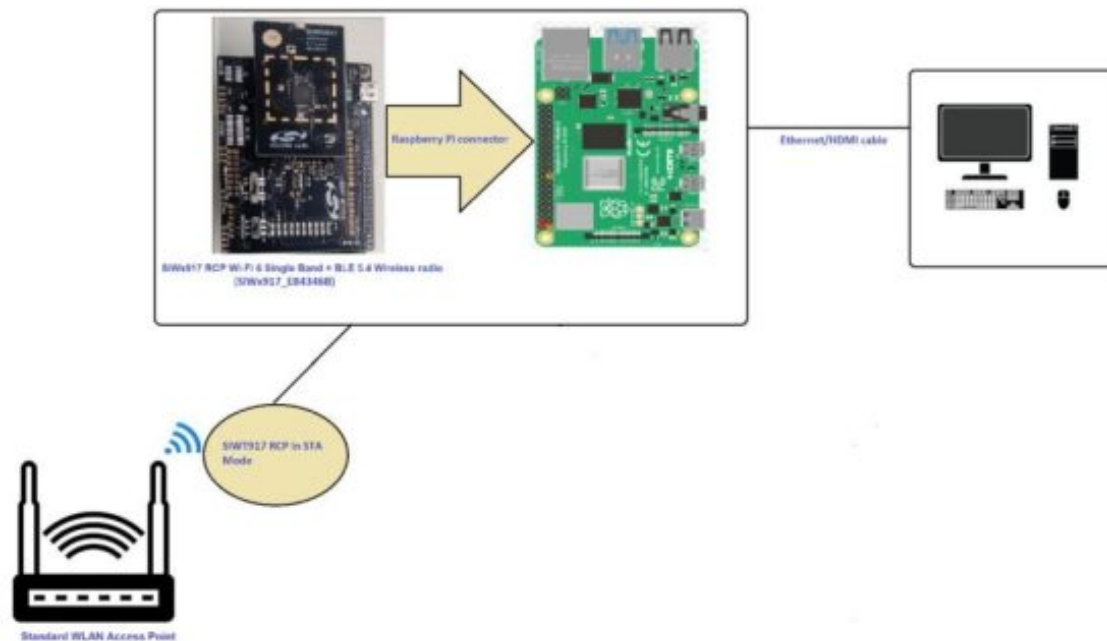
Figure 3.1. Setup Diagram
