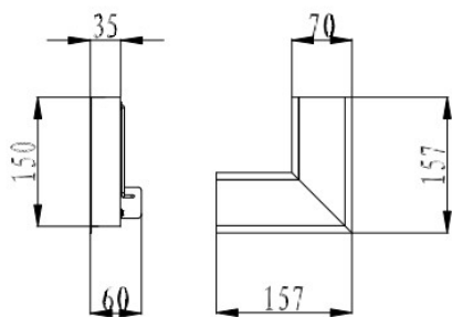
L shape connector-1
