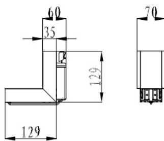
L shape connector-2
