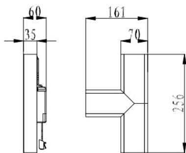
T shape connector
