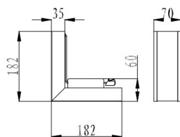
L shape connector-3
