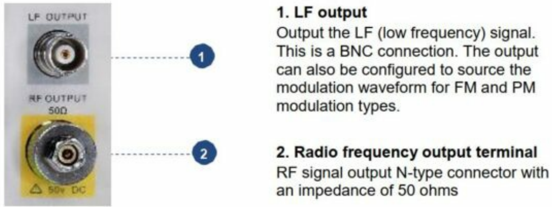
Figure 1-6 Front panel connectors
