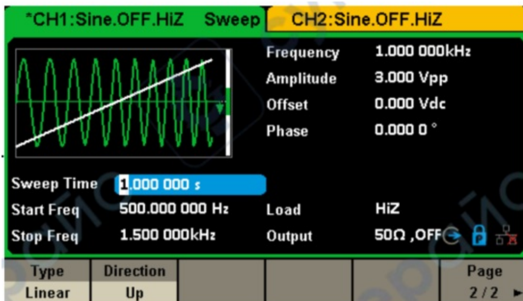
Figure 2-36 Linear Sweep Interface
