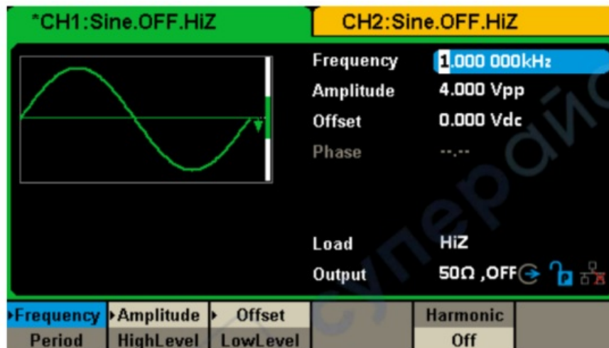
Figure 2-84 Independent Mode
