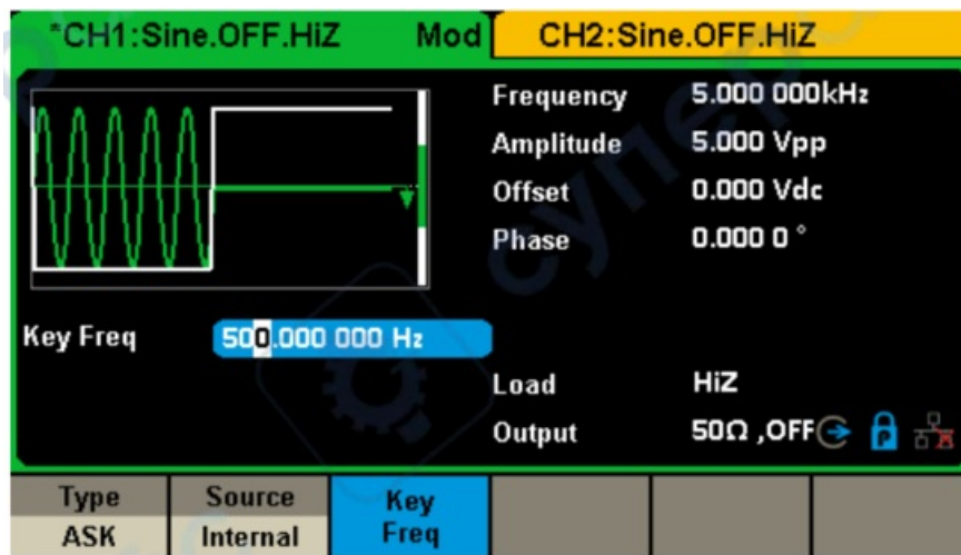
Figure 3-13 Generate an ASK Modulation Waveform
