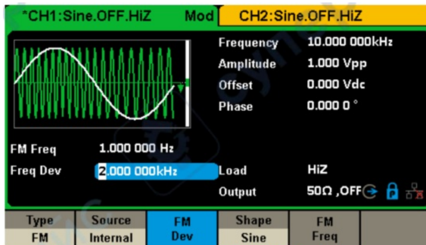
Figure 3-10 Generate a FM Modulation Waveform
