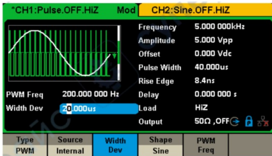
Figure 3-15 Generate a PWM Modulation Waveform
