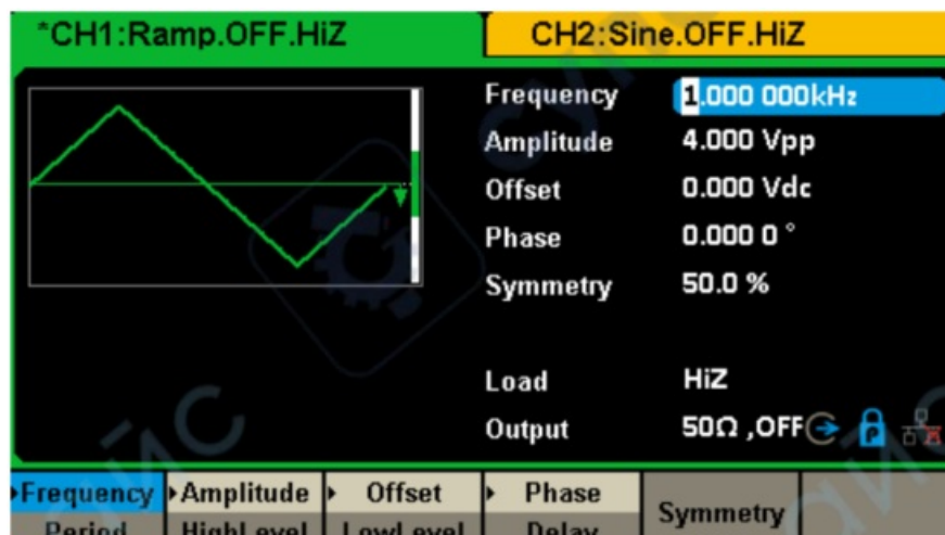
Figure 1-8 Ramp Display Interface
