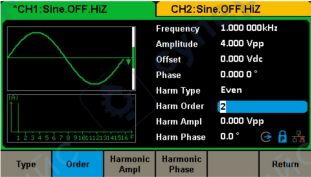
Figure 2-23 Harmonic Interface
