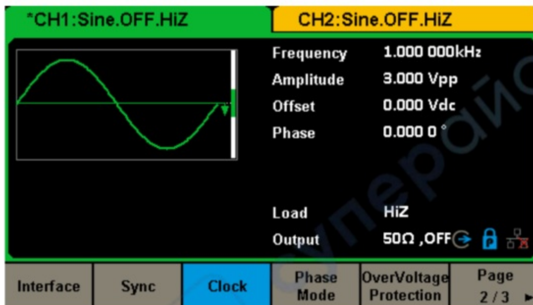
Figure 2-48 Utility Setup Interface (Page 2/3)
