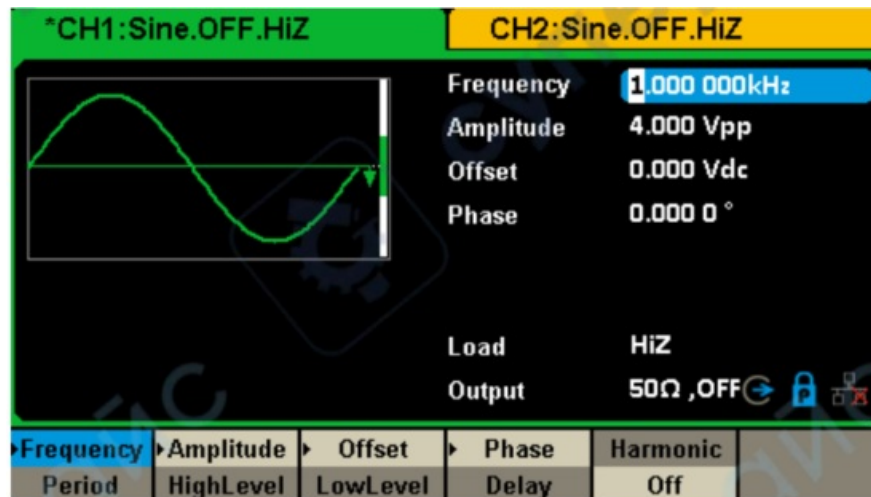
Figure 1-6 Sine Display Interface
