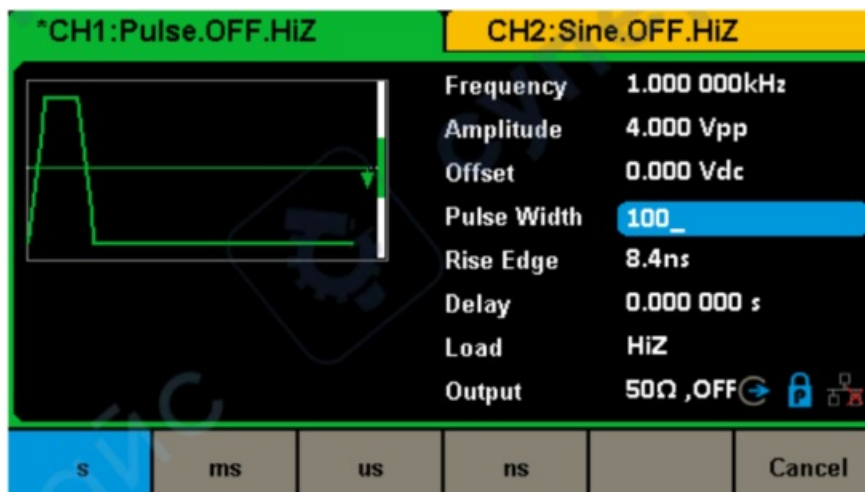
Figure 2-11 Setting the Pulse Width
