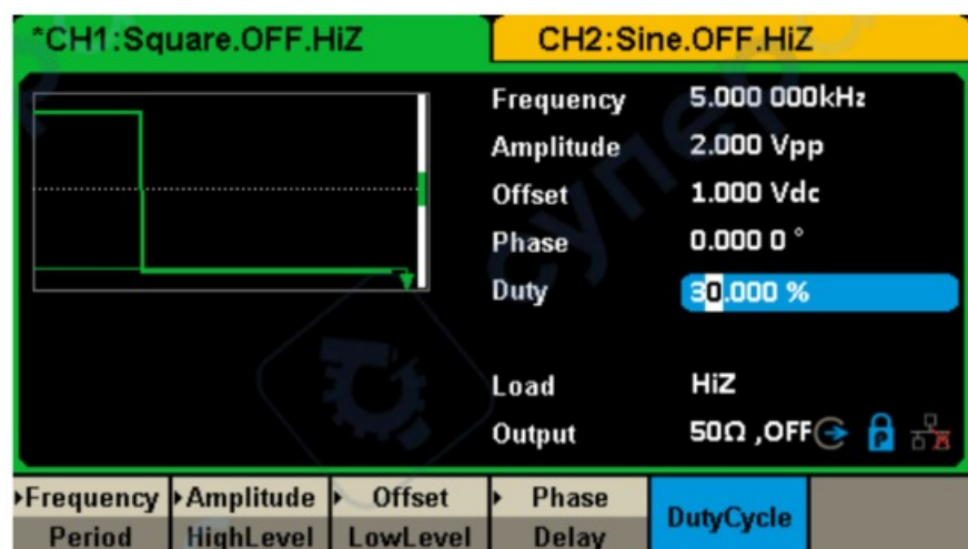
Figure 3-2 Generate a Square Waveform
