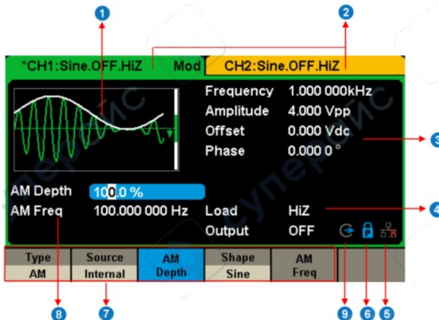
Figure 1-4 Touch Screen Display
