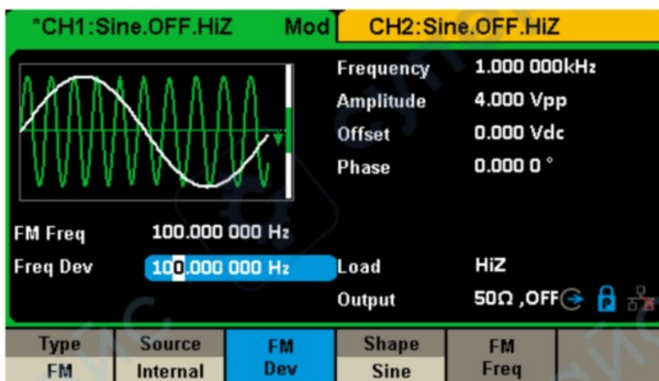
Figure 2-26 Setting Interface of FM Modulation
