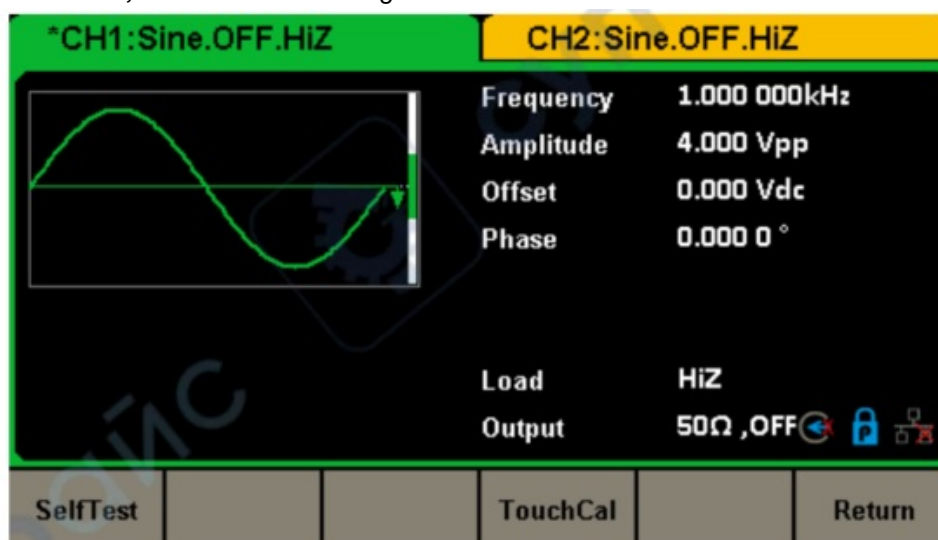
Figure 2-59 Test/Cal function Menu
