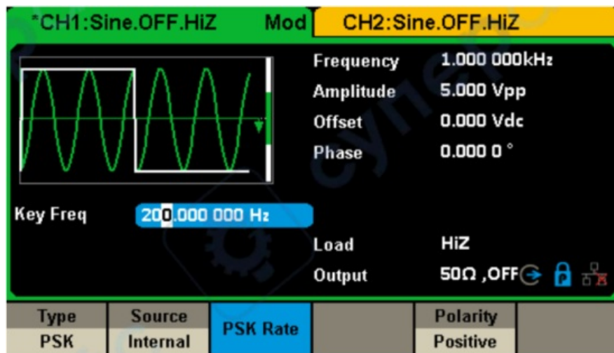
Figure 3-14 Generate a PSK Modulation Waveform
