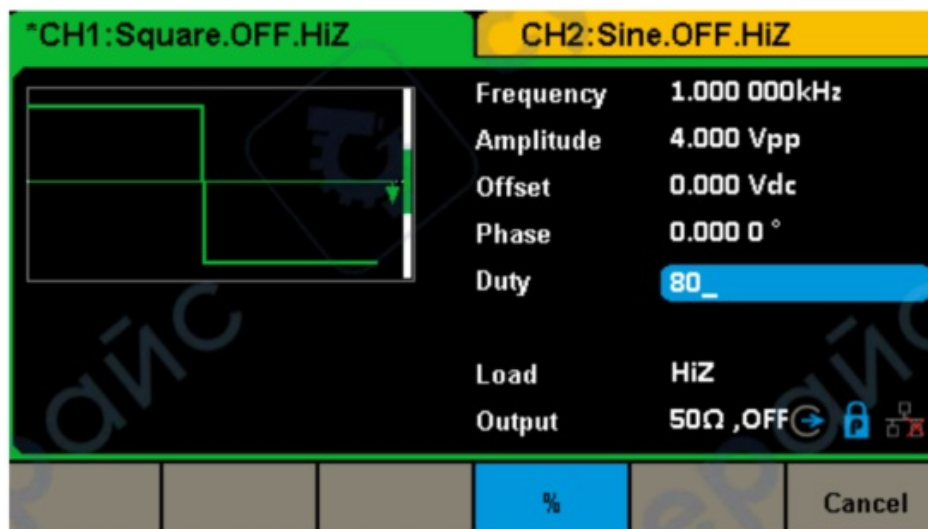
Figure 2-7 Setting the Duty Cycle
