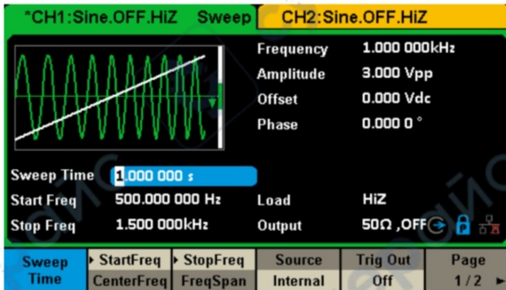
Figure 2-34 Setting Interface of Sweep (Page 1/2)
