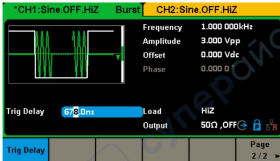
Figure 2-42 Gated Burst Interface (Page 2/2)
