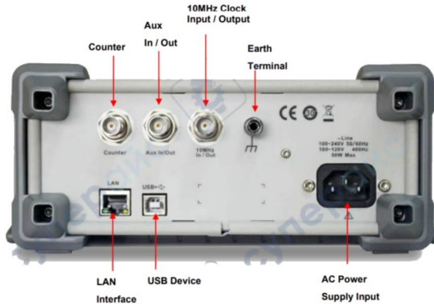
Figure 1-3 Rear Panel of SDG2000X
