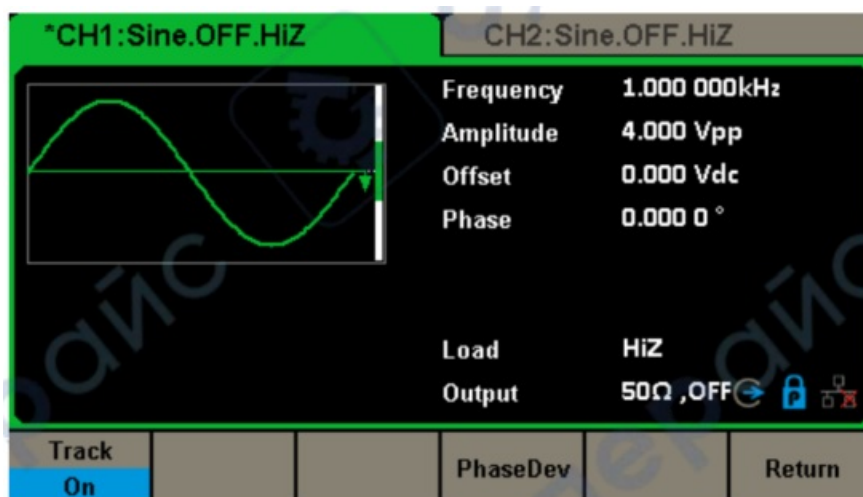
Figure 2-74 Track Interface
