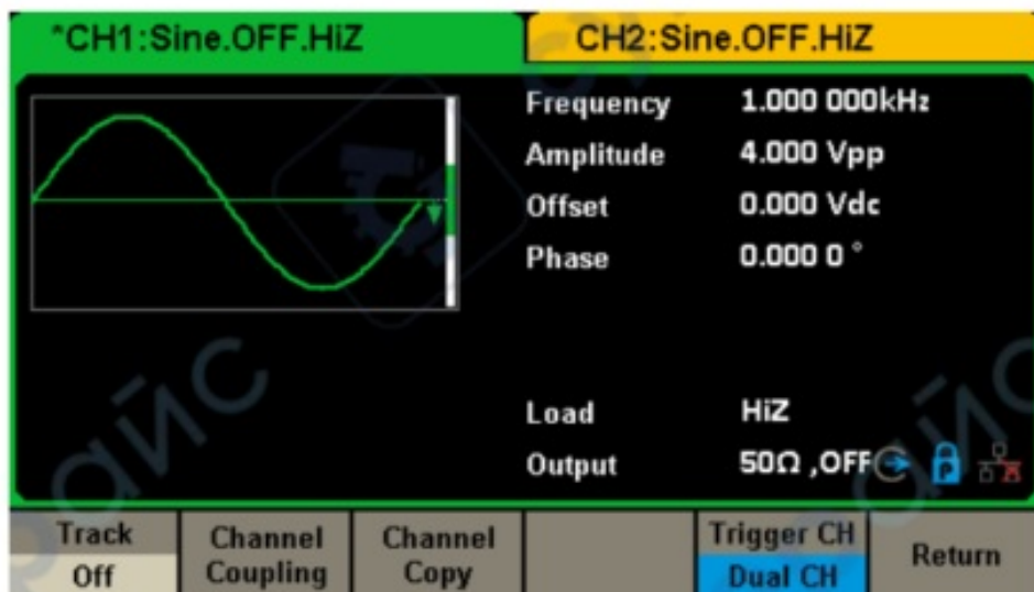
Figure 2-77 Channel trigger signal correlation
