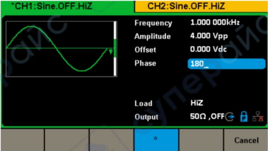
Figure 2-5 Setting the Phase
