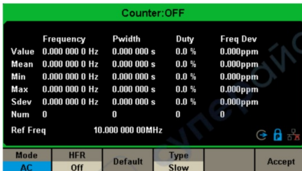
Figure 2-68 Counter Setup Interface
