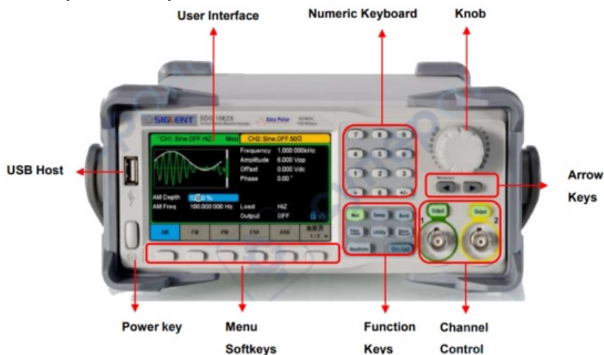
Figure 1-2 Front Panel of SDG2000X
