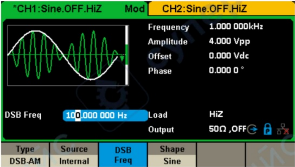
Figure 2-25 Setting Interface of DSB-AM Modulation
