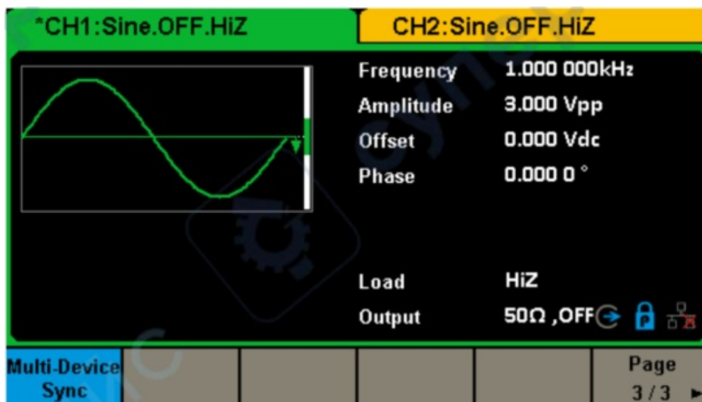
Figure 2-49 Utility Setup Interface (Page 3/3)
