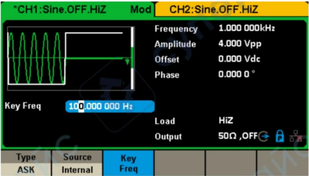
Figure 2-29 Setting Interface of ASK Modulation
