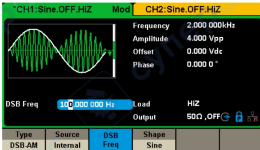
Figure 3-16 Generate a DSB-AM Modulation Waveform
