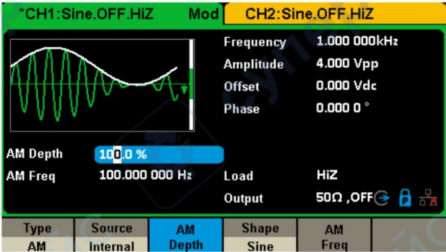
Figure 1-14 Modulation Display Interface
