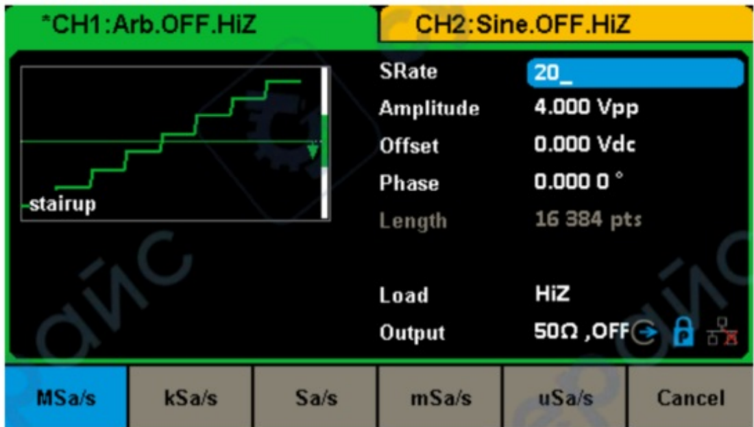
Figure 2-20 Setting the Sampling Rate
