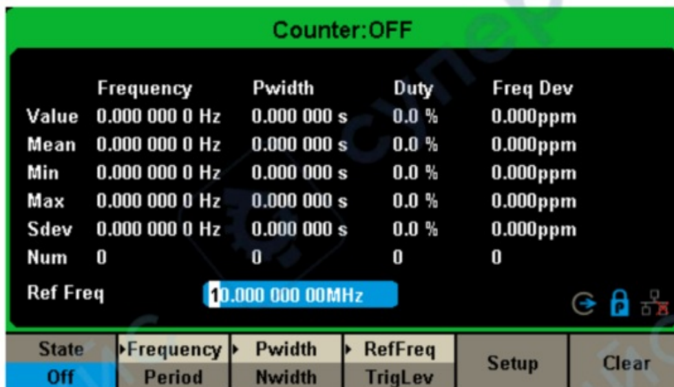
Figure 2-67 Frequency Counter Interface
