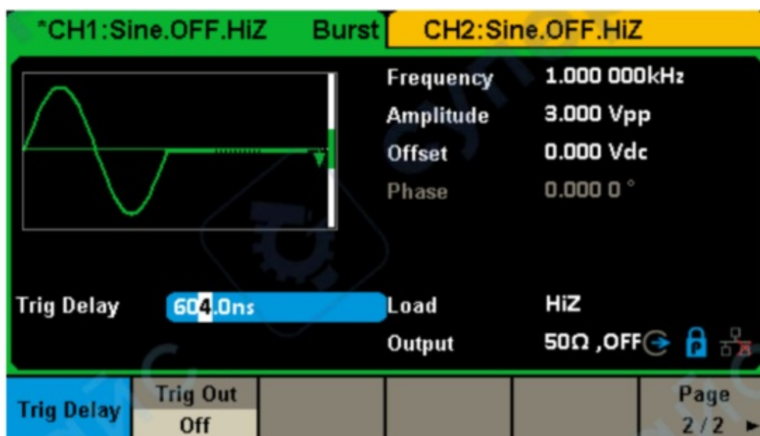
Figure 2-39 N-Cycle Burst Interface (Page 2/2)
