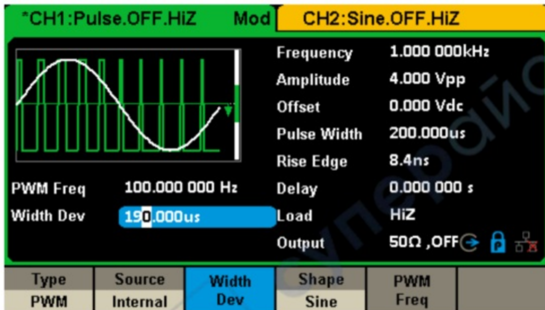
Figure 2-31 Setting Interface of PWM Modulation
