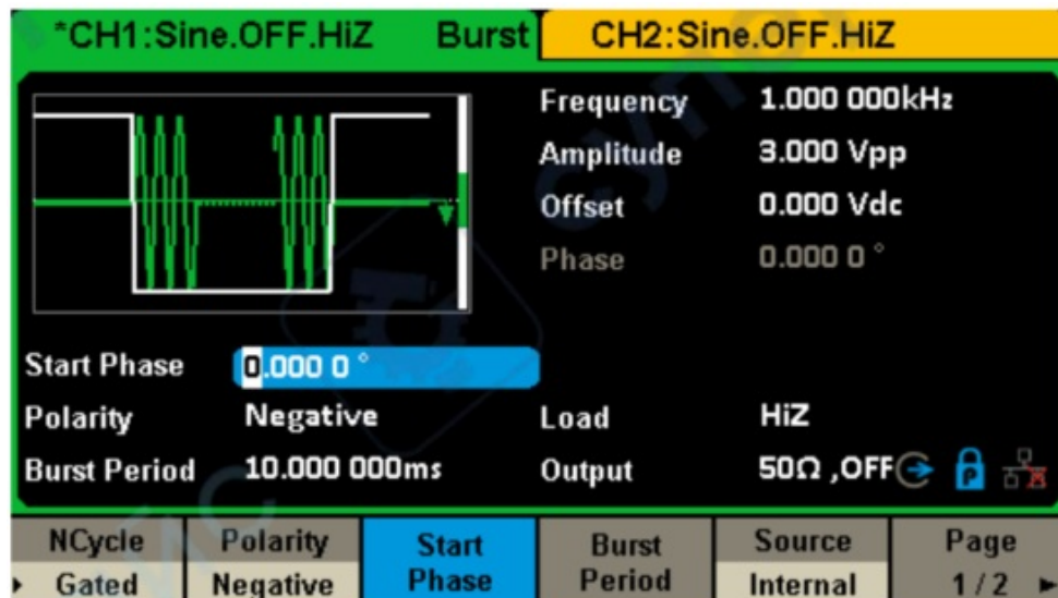
Figure 2-41 Gated Burst Interface (Page 1/2)
