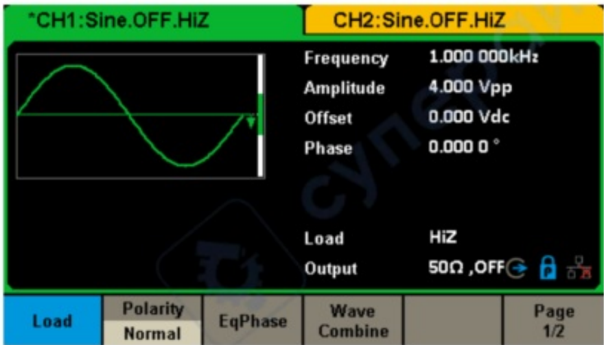
Figure 2-69 Output Setup Interface
