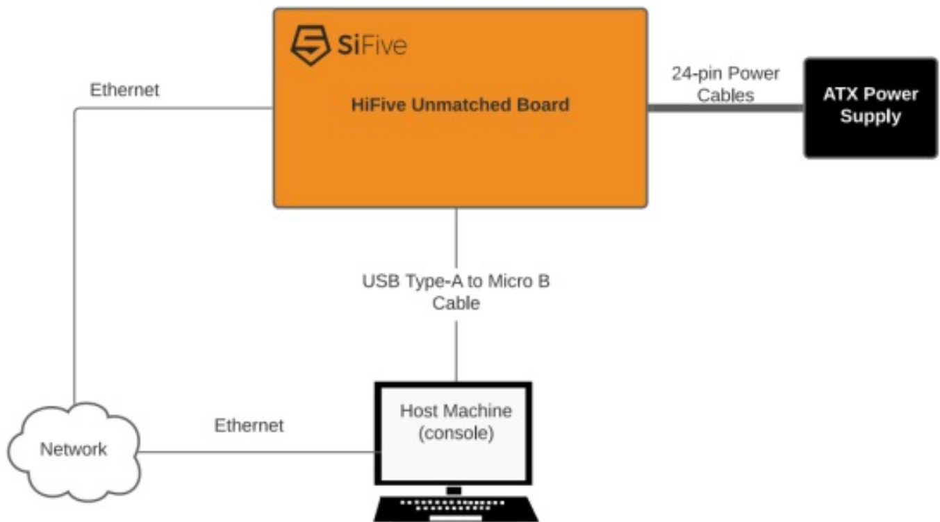
Figure 3: HiFive Unmatched System Block Diagram
