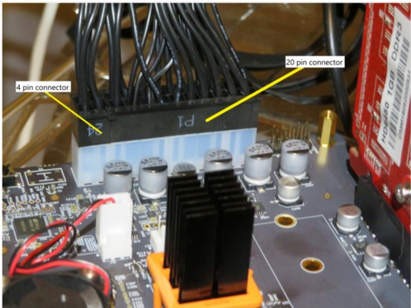
Figure 6: ATX Connection
