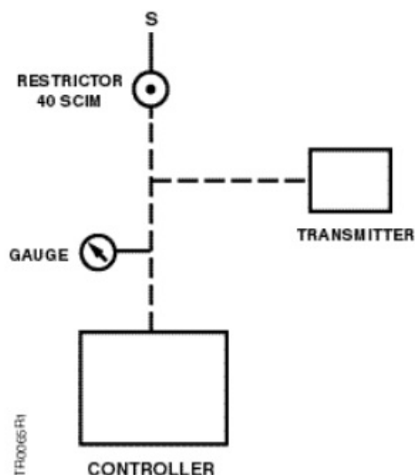
Figure 8. Typical Connections.
