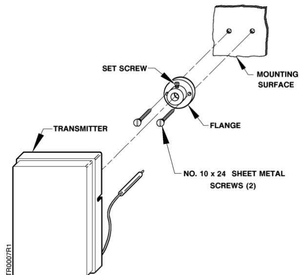
Figure 5. Remote Bulb Mounting.
