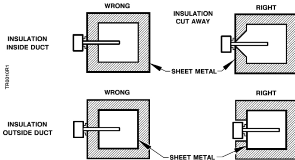
Figure 3. Installation on Insulated Ducts.
