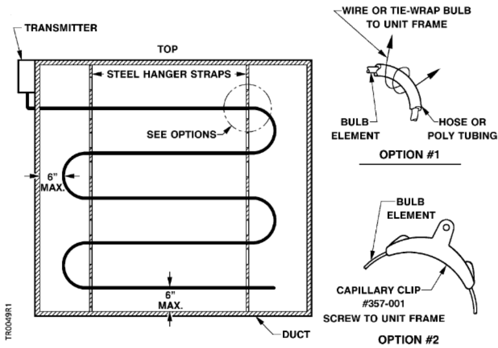
Figure 4. Mounting the Averaging Bulb in Large Ducts.
