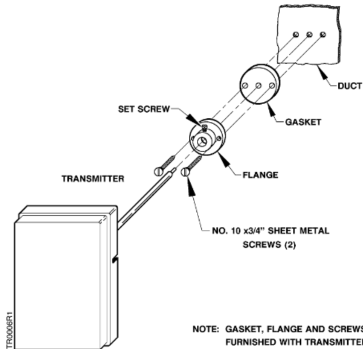
Figure 2. Rigid Bulb Mounting.
