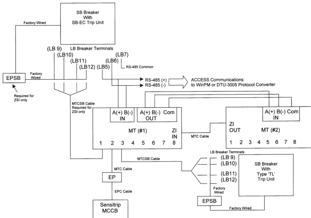
Figure 1 – System Connection Diagram
