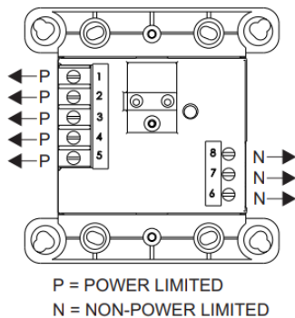
Figure 5 HTRI-RZ Power Limited Wiring
