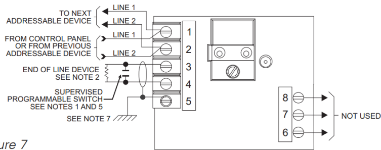
Figure 7 HTRI-SZ Wiring
