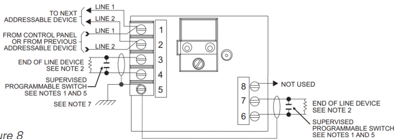
Figure 8 HTRI-DZ Wiring
