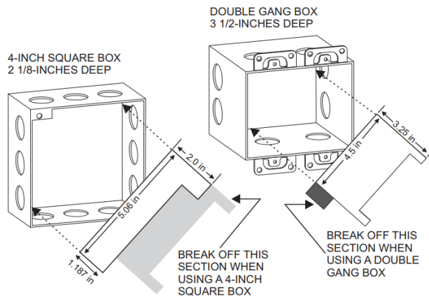
Figure 4 Installing the HTRI-RZ Control Module Barrier
