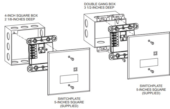
Figure 10 Mounting the HTRI-SZ/-RZ/-DZ
