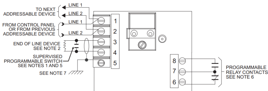
Figure 6 HTRI-RZ Wiring
