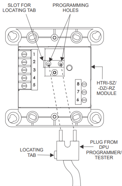
Figure 2 Connecting The DPU Plug
