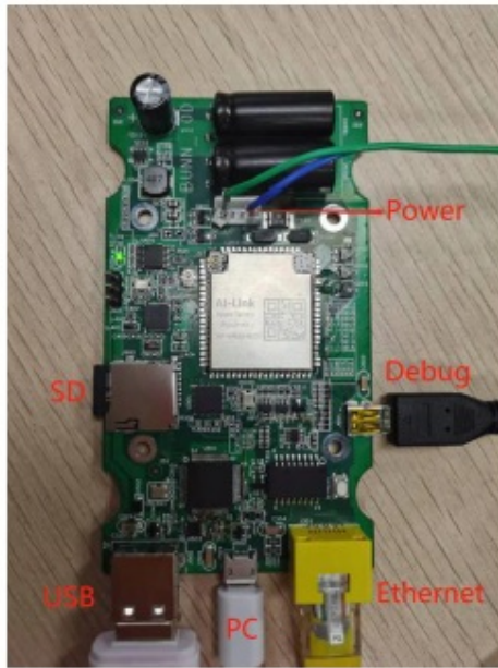
Figure 1. Device interfaces
