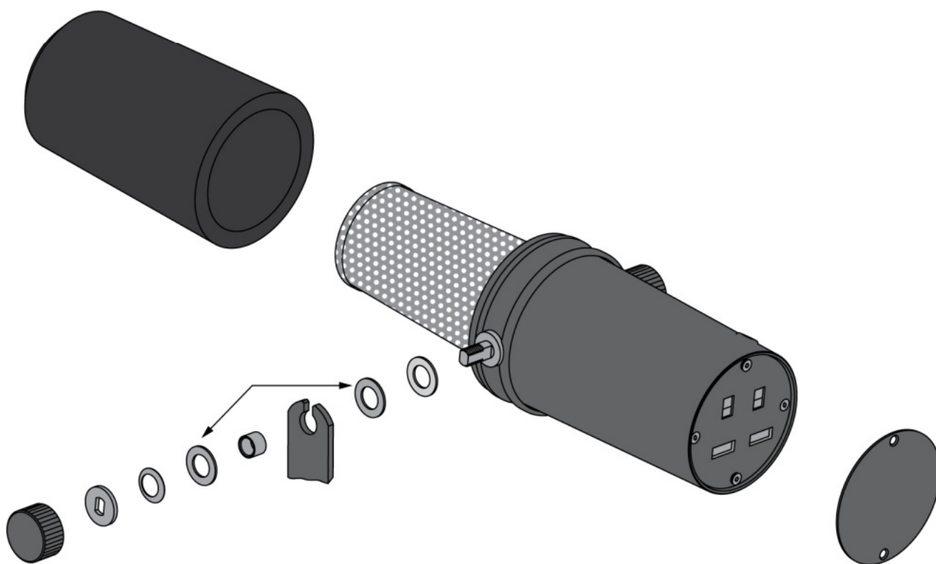
Mounting Assembly - Exploded View
