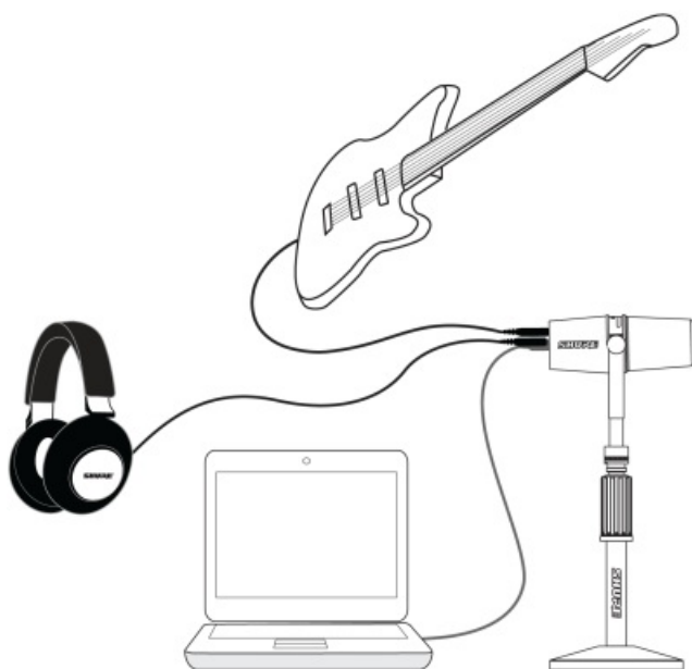
Connecting a ¼" TS/TRS Input
