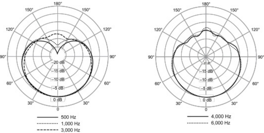
Typical Polar Pattern
