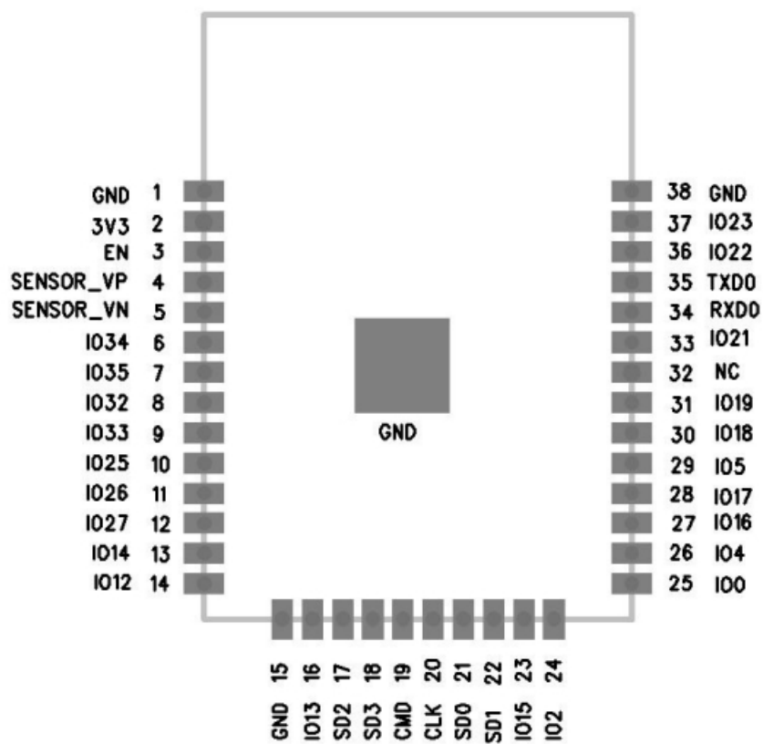
ESP32-SL PIN definition diagram
