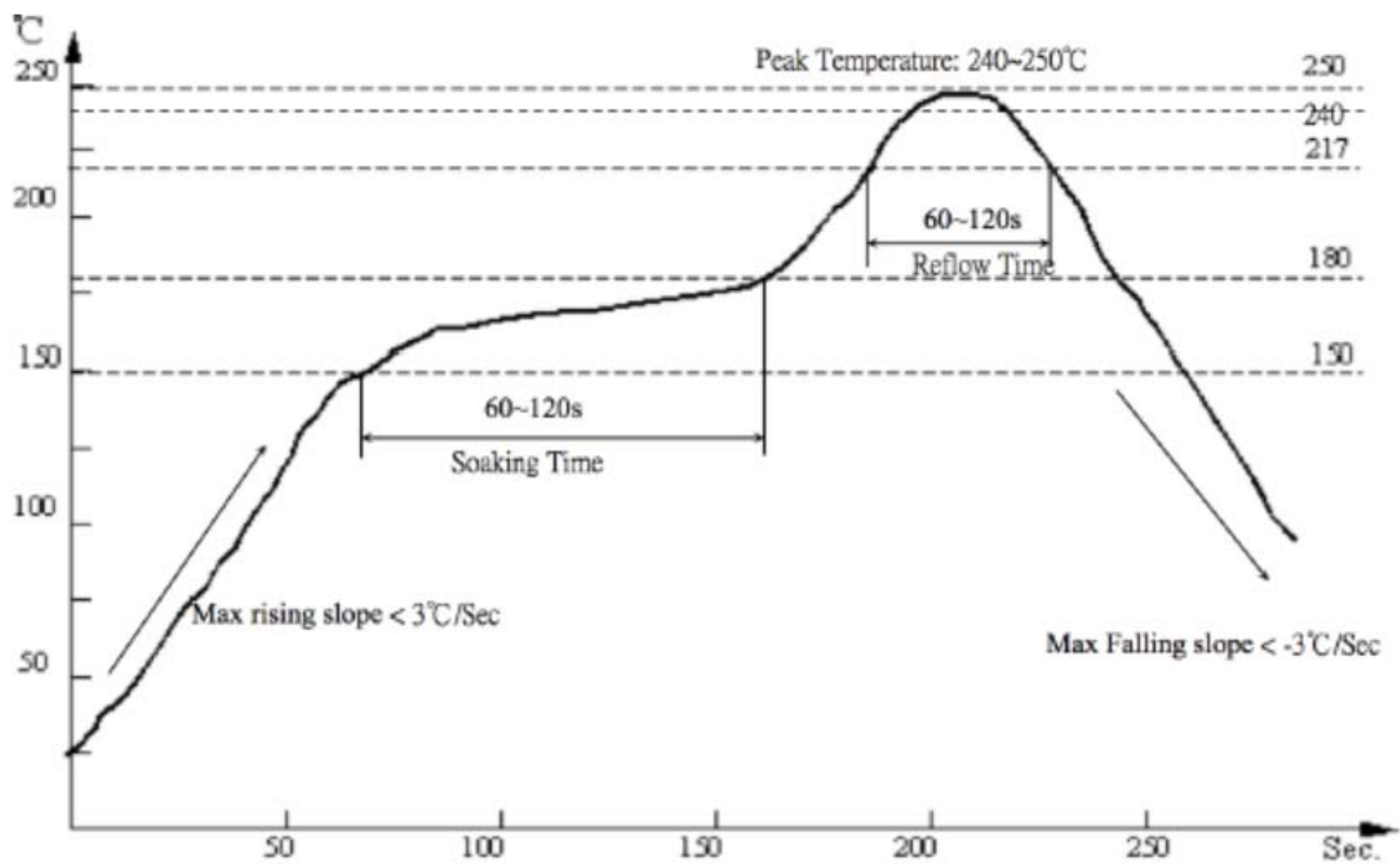
Fig.8.1 Recommended Reflow Profile
