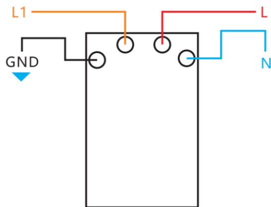
1 gang switch
