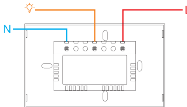
Dimmer switch
