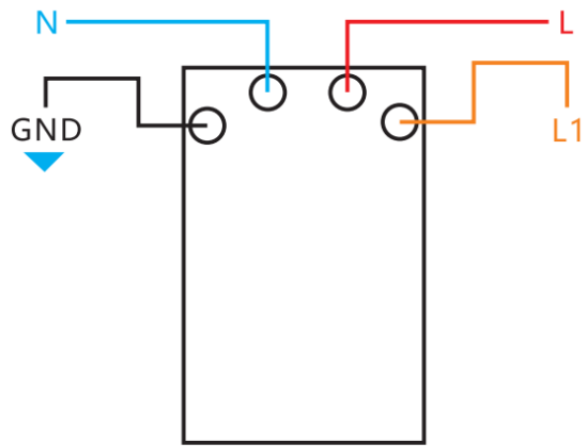
Dimmer switch
