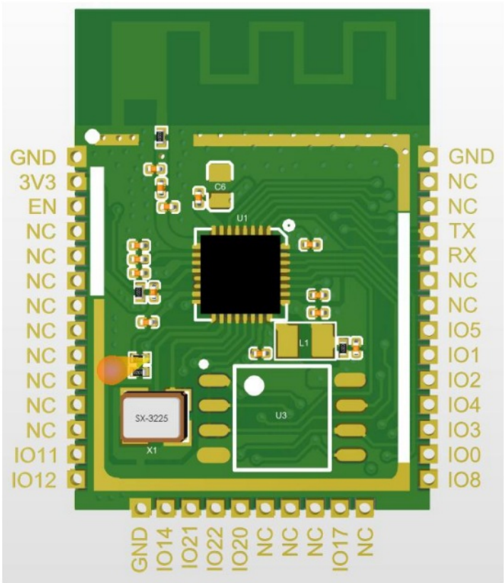
2.1 Figure 2.1 BL-61C Pin diagram
