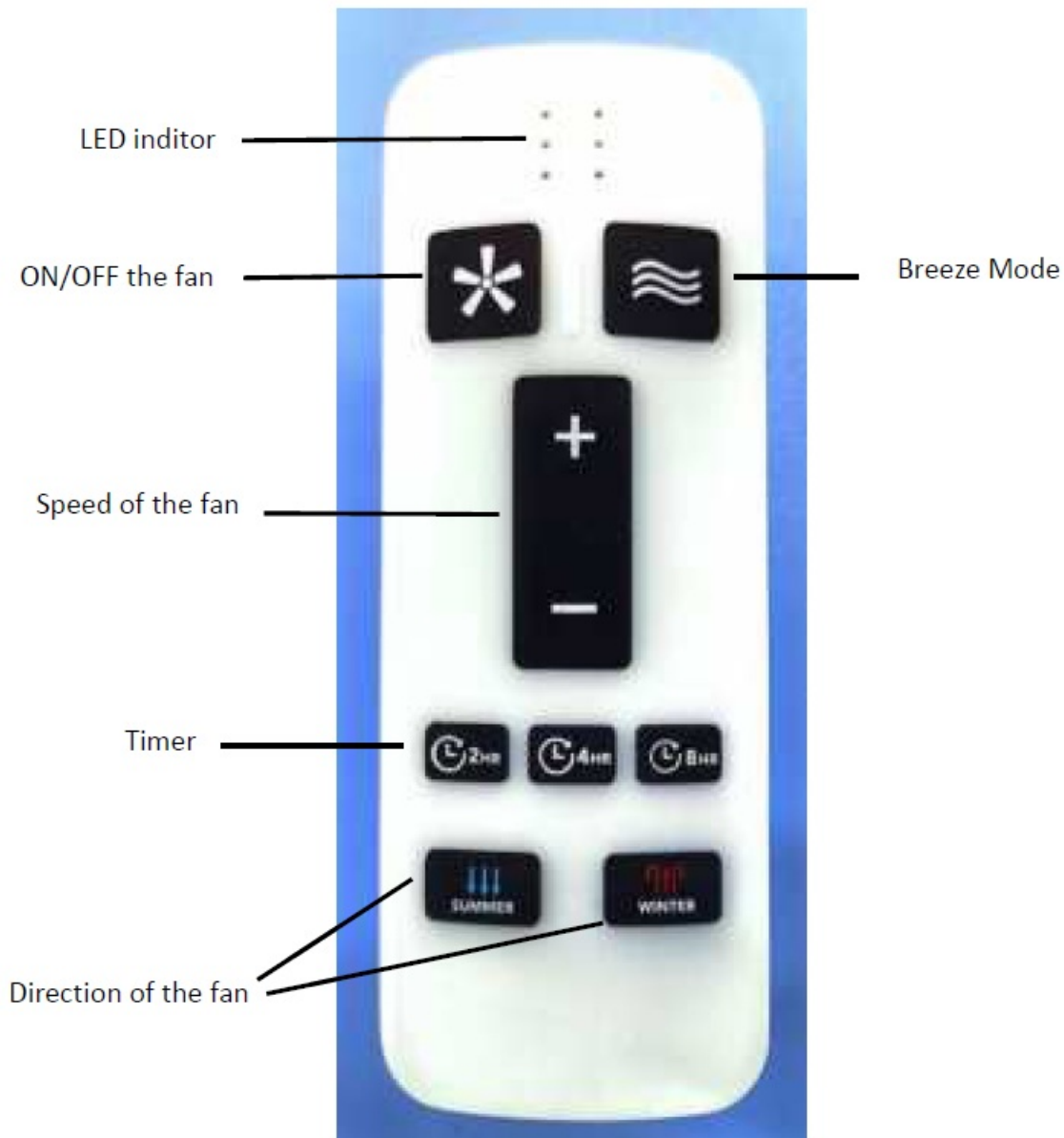
FT0309HD transmitter
