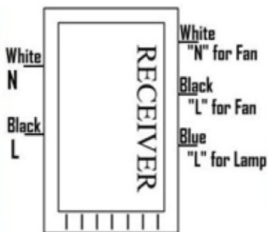
Wiring Diagram of Receiver
