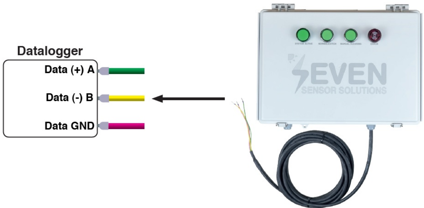
Figure 22 – Communication Cable Connection
