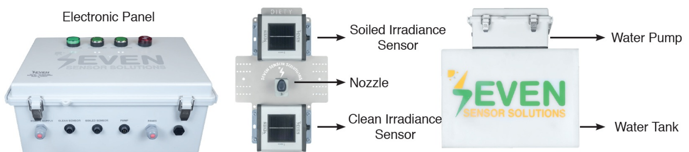
Figure 1 – Components of the Automatic Soiling Sensor
