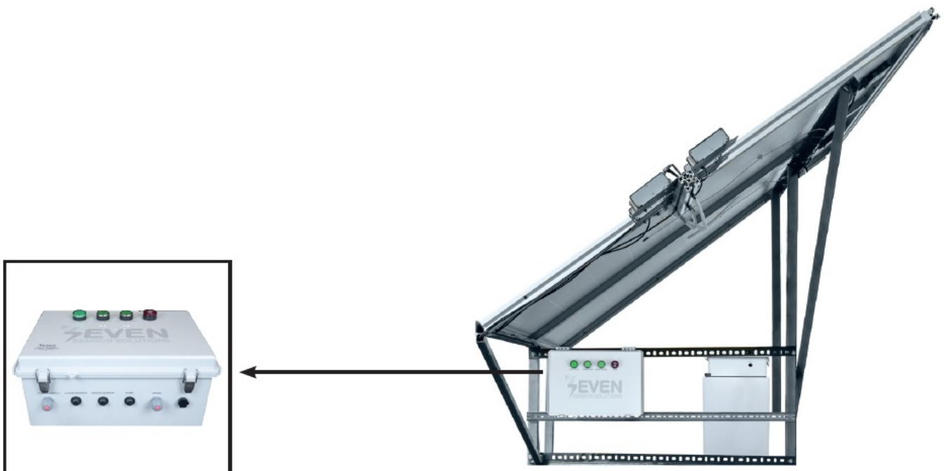
Figure 9 – Installation of the Electronic Panel
