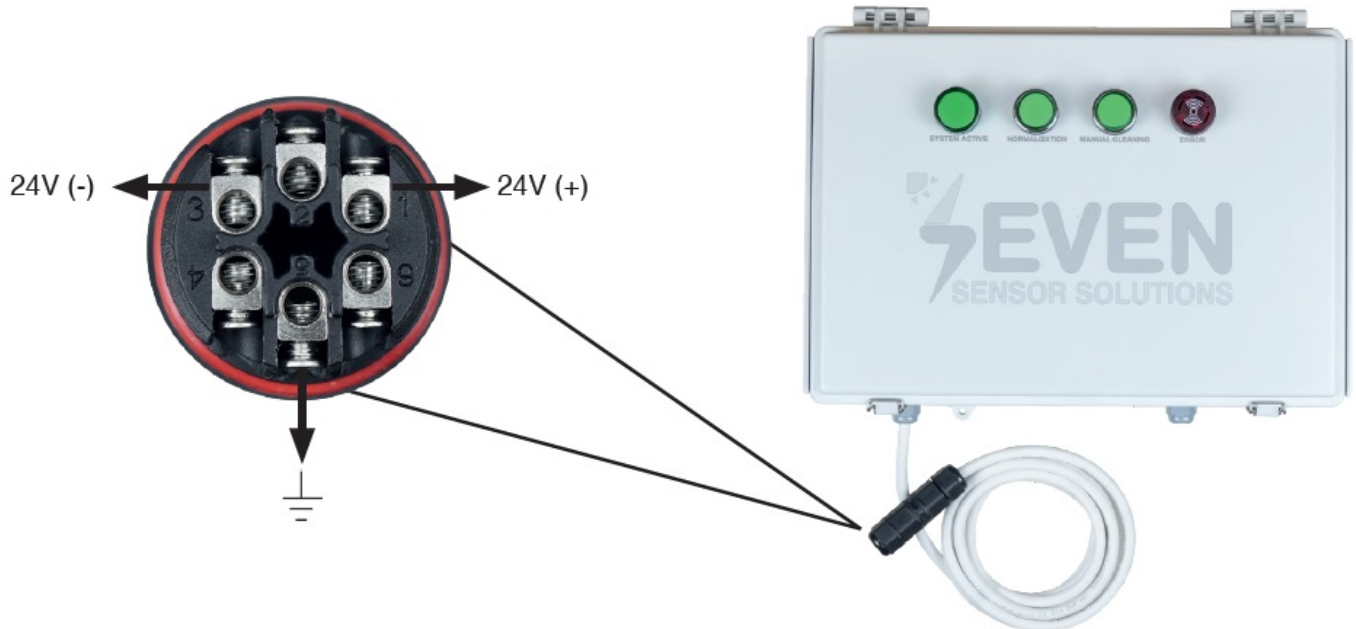
Figure 14 – 24V Power Cable Connection
