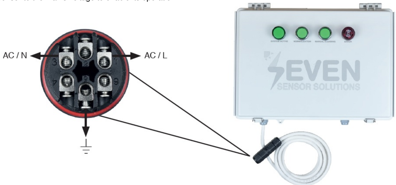
Figure 13 – Connection of the Power Cable
