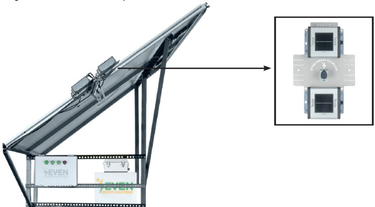
Figure 6 – Installation of Irradiance Sensors
