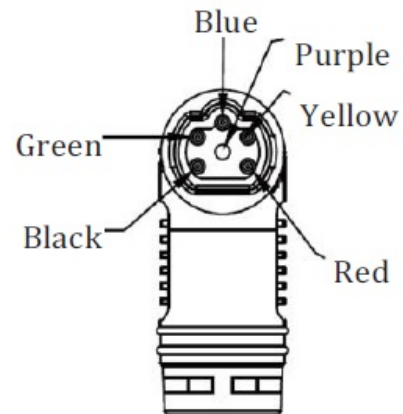
6P cable connector (Male)
