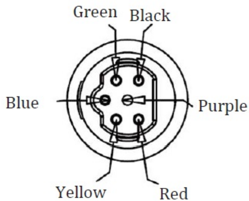
6P Cable Connector (Female)
