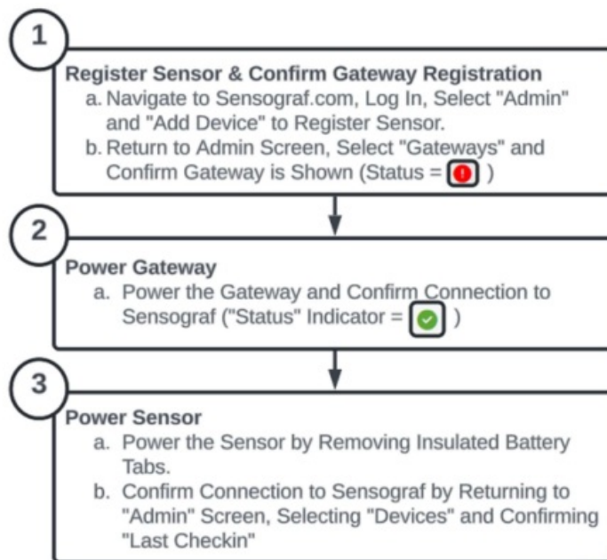
Figure 4: Step-by-Step Process to Install and Register Sensograf-Supplied Sensor, Gateway, and Platform
