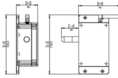
Drawing 2: Housing with Attached RH/Temp Probe
