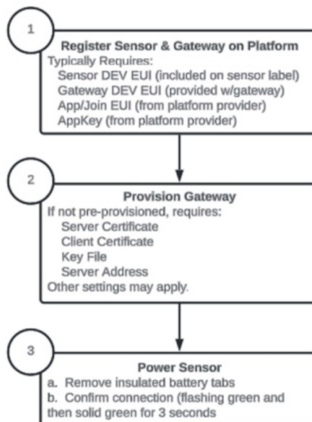
Figure 5: Step-by-Step Process to Install and Register Sensograf-Supplied Sensor with 3rd Party Gateway, & Platform
