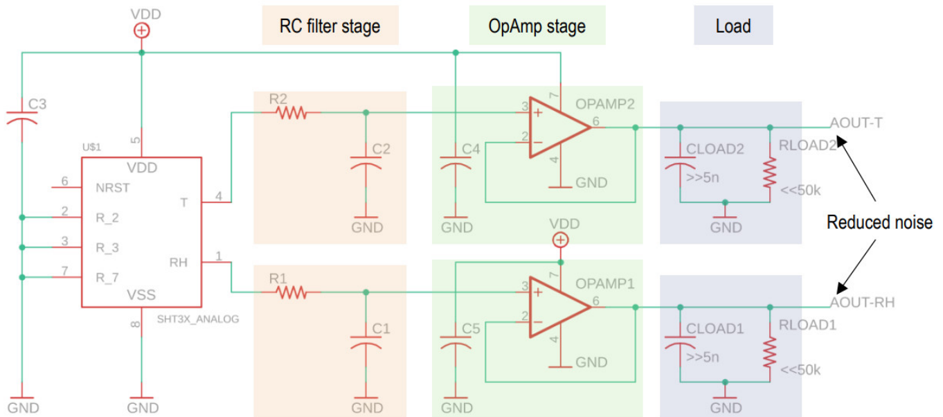
Figure 4. Possible improved schematic for the SHT3x. This solution allows greater drive capability and reduces output noise.
