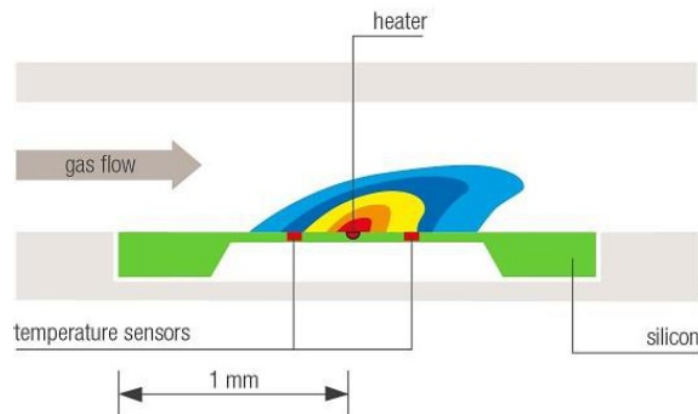
Figure 1. Cross-section view of the gas channel.
