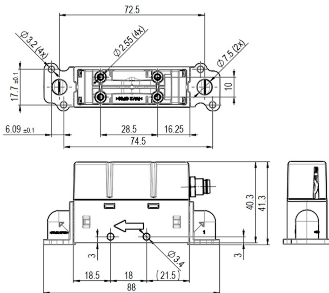
Figure 9. Physical dimensions and mounting information for SFC6000D with downmount fittings. All units are in [mm].
