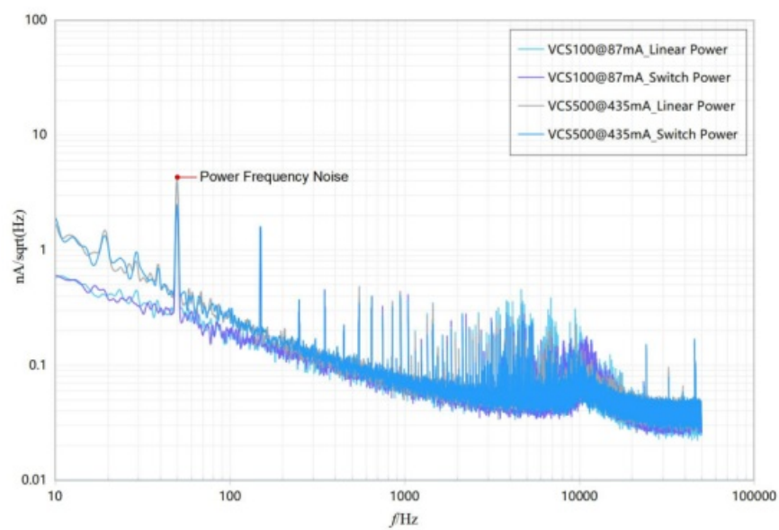
Figure6 Current Noise Spectral Density Plot of VCS
