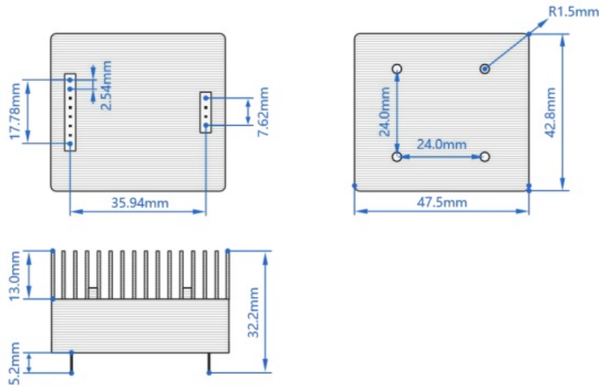
Figure5 Dimensional drawing of VCS250/500/1000
