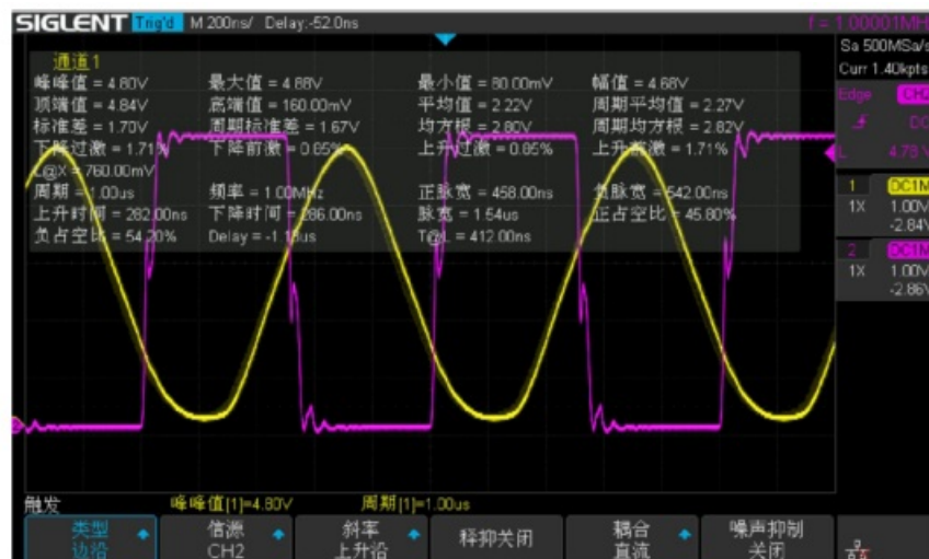
Figure9 Modulation Depth Test Graph
