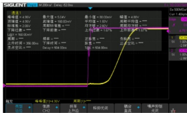
Figure7 Rise Time Test Graph
