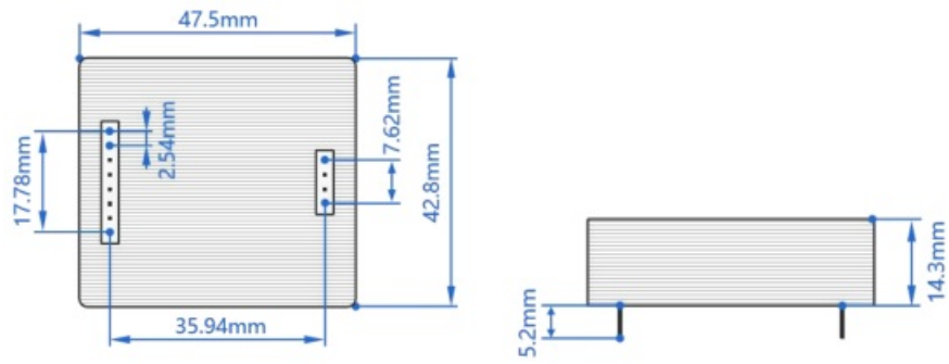
Figure4 Dimensional drawing of VCS100
