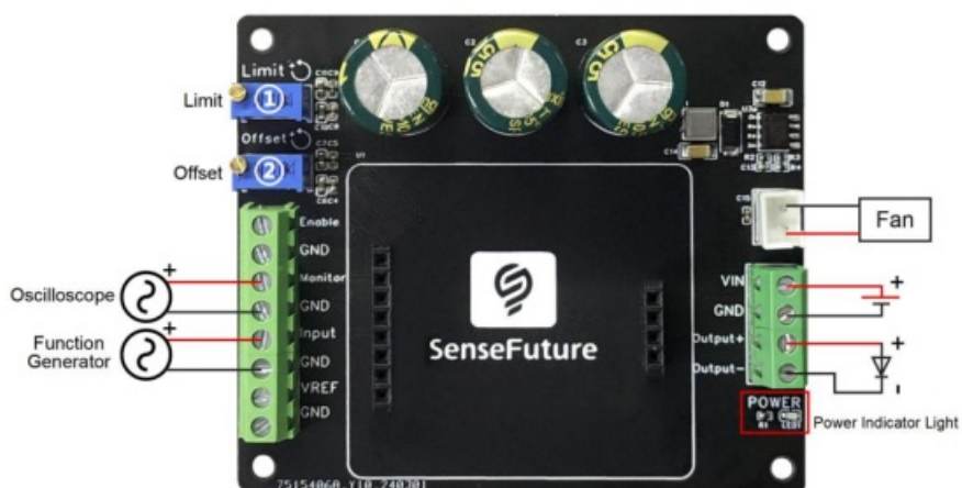
Figure3 Wiring Diagram of VCS Adapter Board
