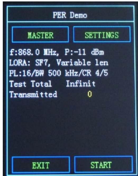
Figure 7: PER Demo Master Display
