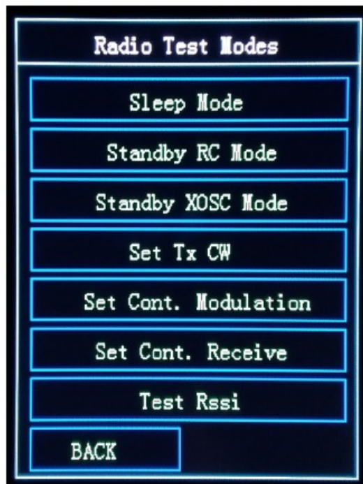
Figure 8: Radio Test Modes Display
