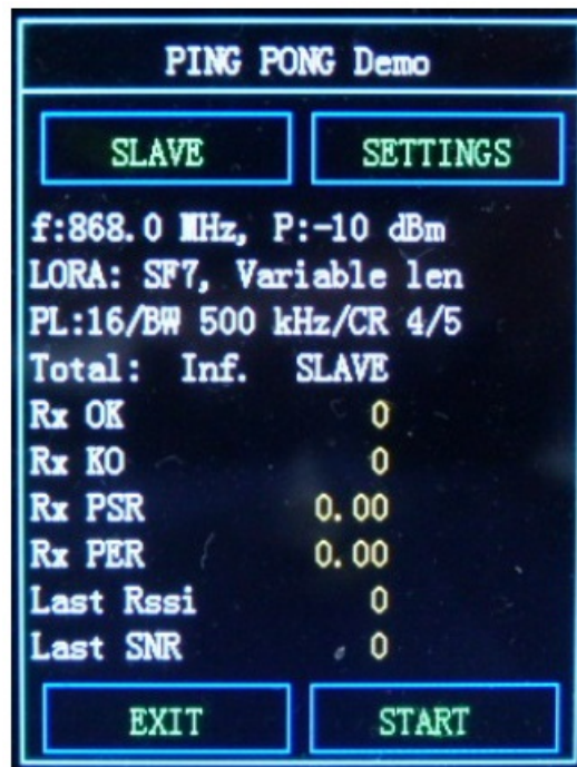
Figure 4. PING PONG Demo Slave Display
