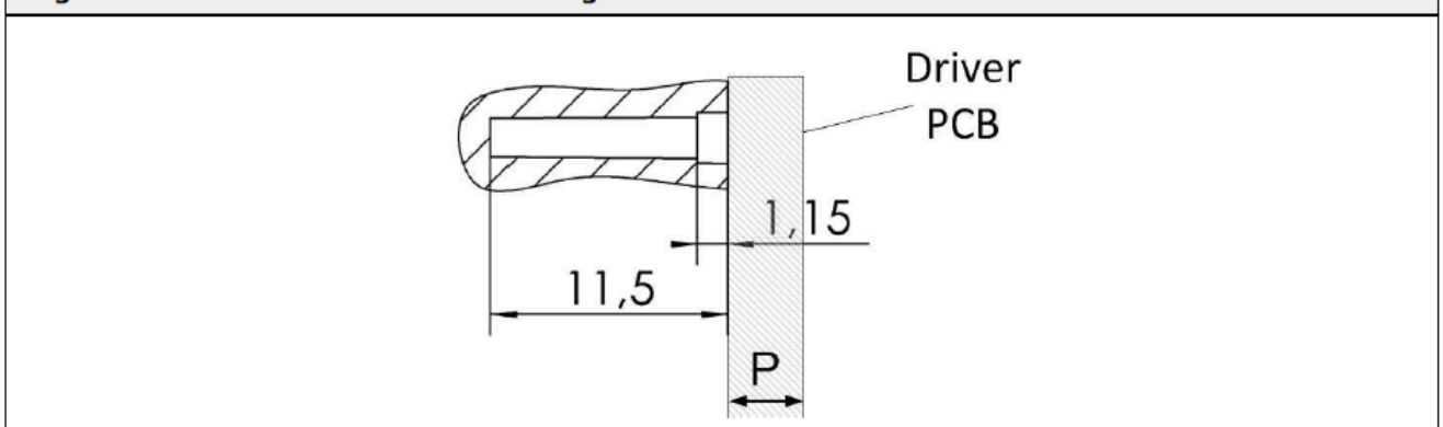
Figure 10: Cross section of a mounting dome with driver PCB
