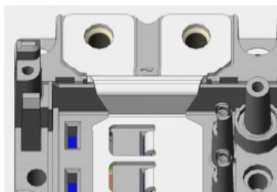
Figure 8: Detail: AC terminal of SKiM
