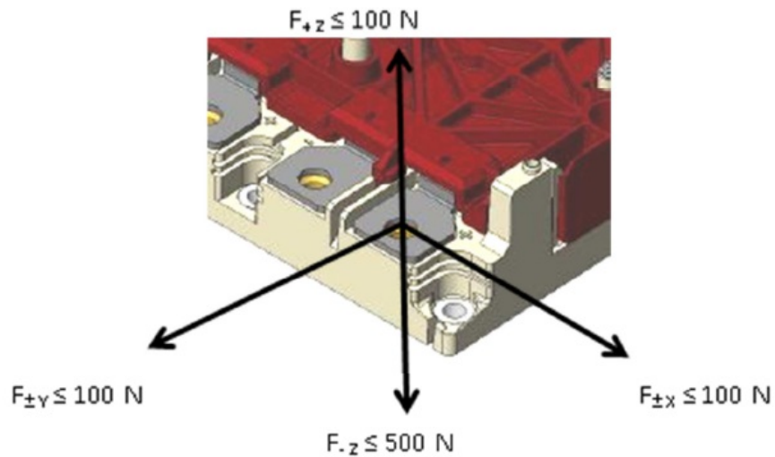
Figure 7: Maximum forces at the main terminals
