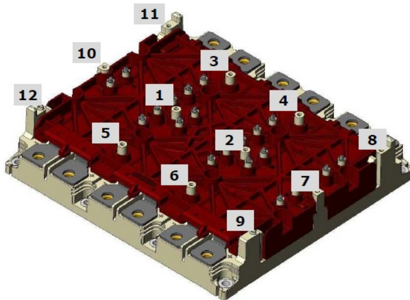
Figure 12: Assembly order for the driver PCB screws
