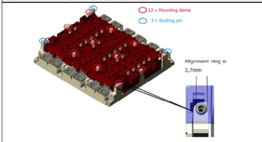
Figure 9: SKiM mounting domes and guiding pins
