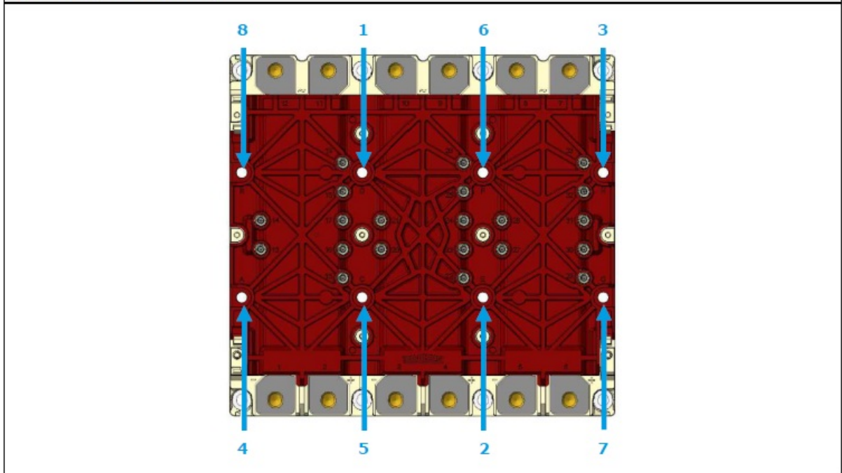
Figure 3: Assembly order for screws for the pressure part of SKiM modules (assembly to heat sink)
