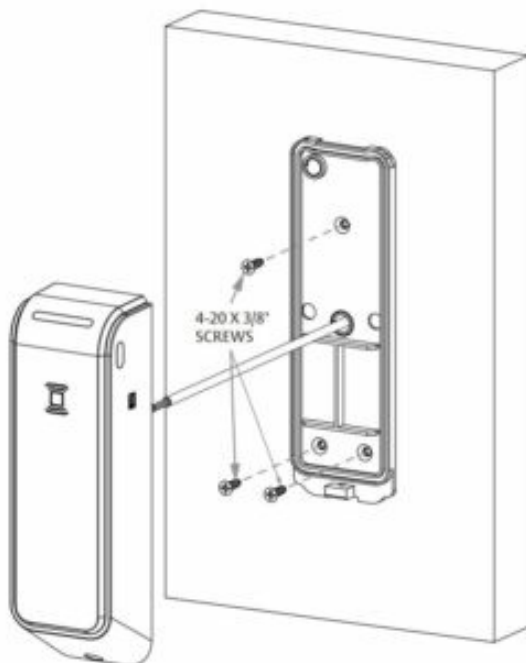
Diagram 15 Secure Reader Backplate.
