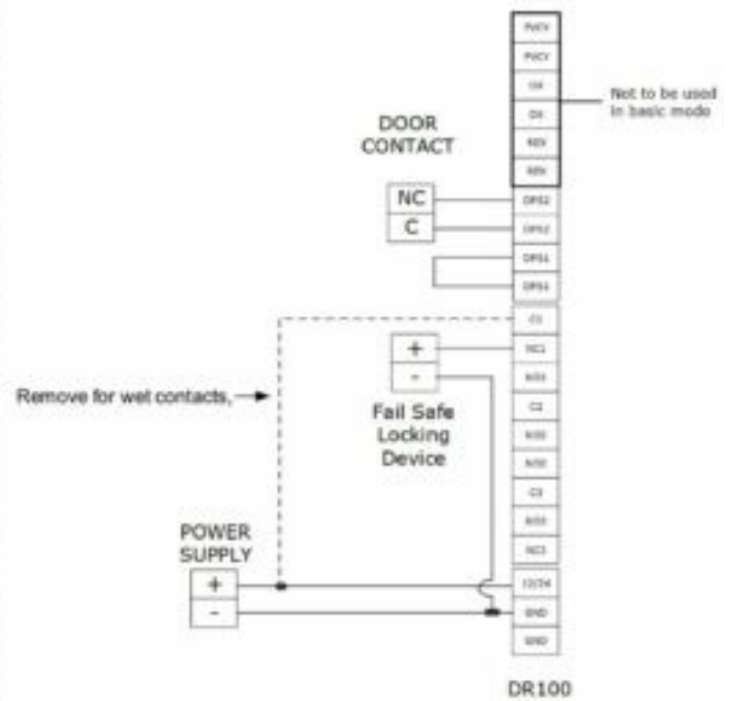
Diagram 6 Typical door system with FAIL-SAFE electric lock.
