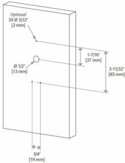
Diagram 12 Drill holes.
