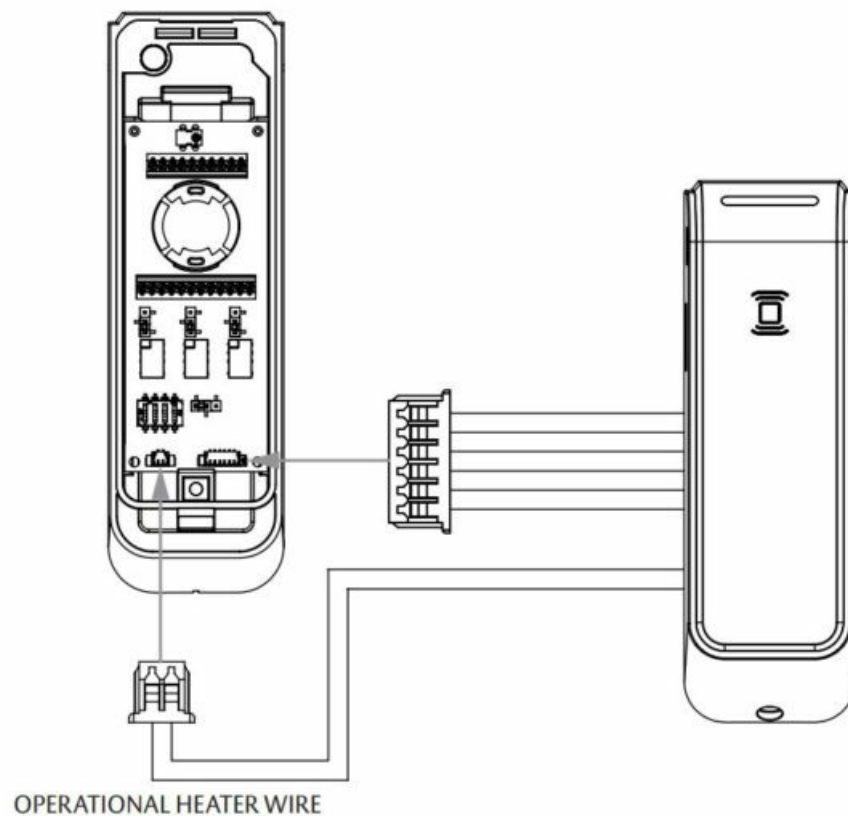
Diagram 10 Hook Reader and install Torx Screw.
