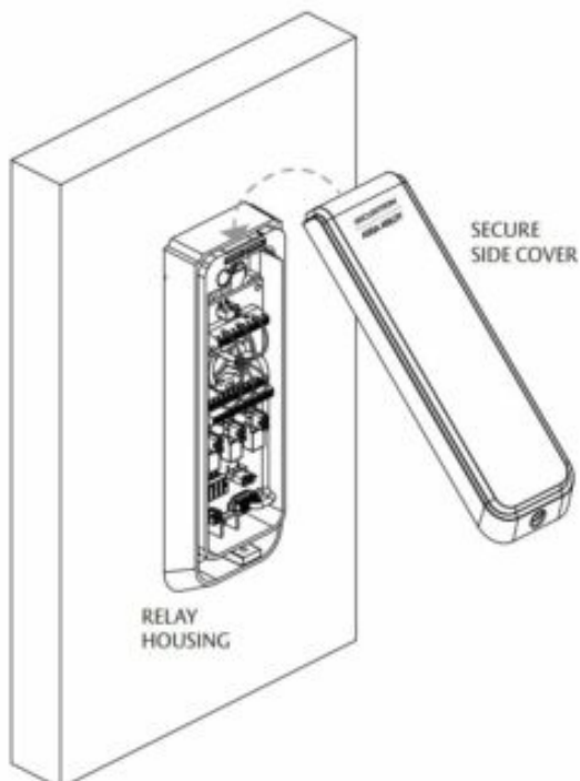
Diagram 19 Secure Side Cover.
