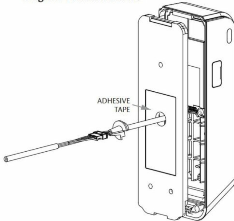
Diagram 14 Mount Reader.
