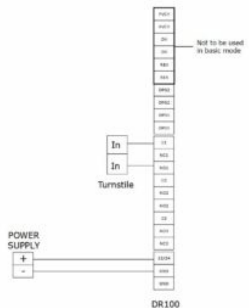
Diagram 8 Typical door system with electronically activated turnstile.
