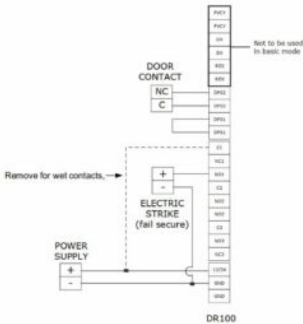
Diagram 5 Typical door system with FAIL-SECURE electric lock.
