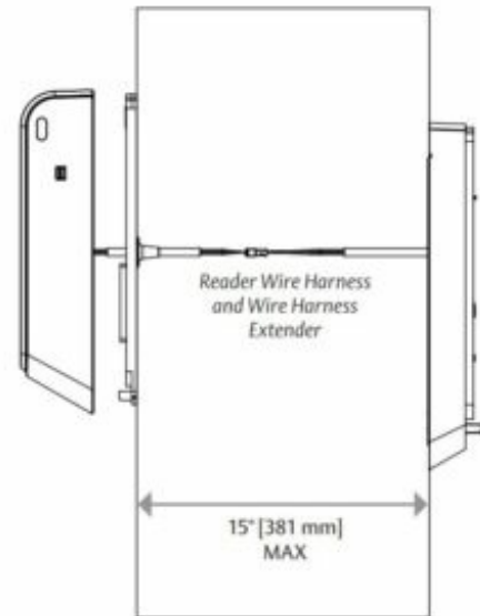
Diagram 13 Route wires.
