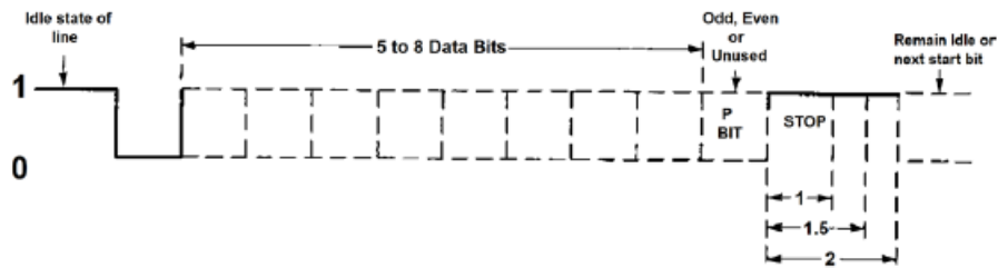
Figure 3 - Asynchronous Communications Bit Diagram
