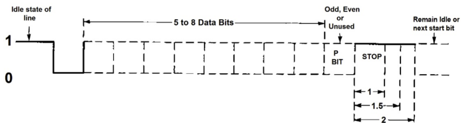
Asynchronous Communications Bit Diagram
