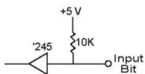
Input Circuit Schematic
