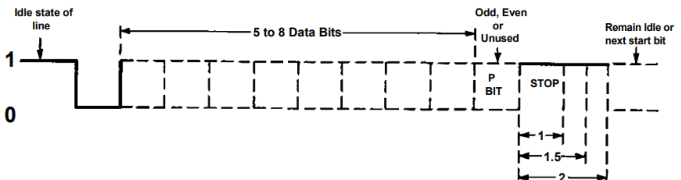
Asynchronous Communications Bit Diagram
