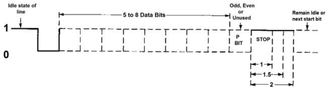
Figure 5 - Asynchronous Communications Bit Diagram
