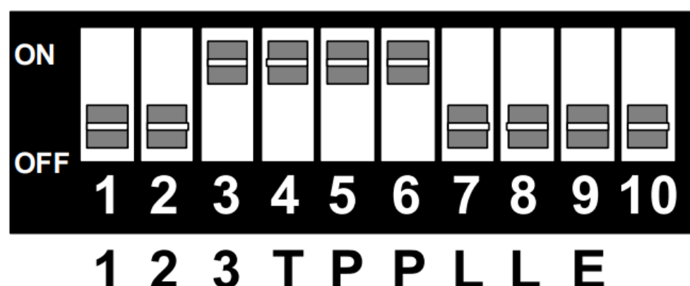
Figure 2 – RS-422
