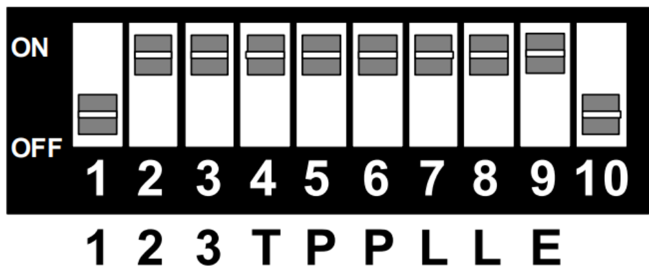
Figure 5 - RS-485, 2-wire without Echo
