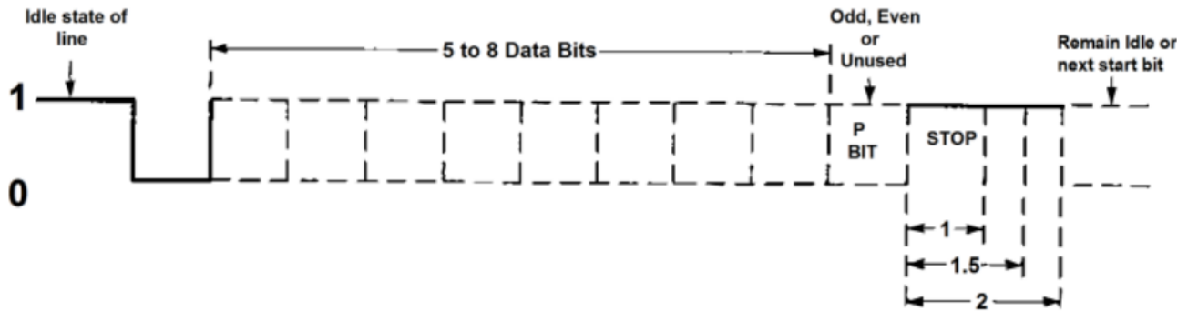
Figure 9 - Asynchronous Communications Bit Diagram
