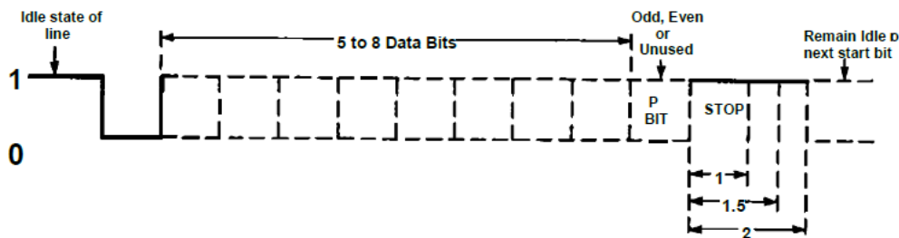
Figure 3 - Asynchronous Communications Bit Diagram
