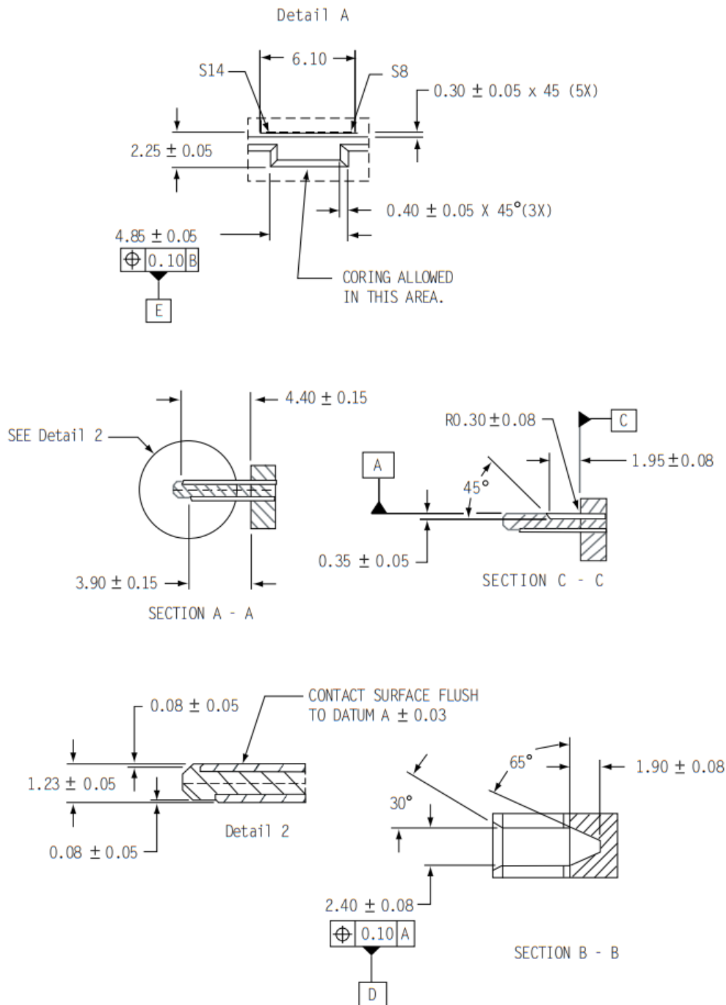
Figure 10. SAS device plug dimensions (detail)
