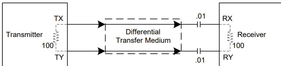
Figure 11. SAS transmitters and receivers
