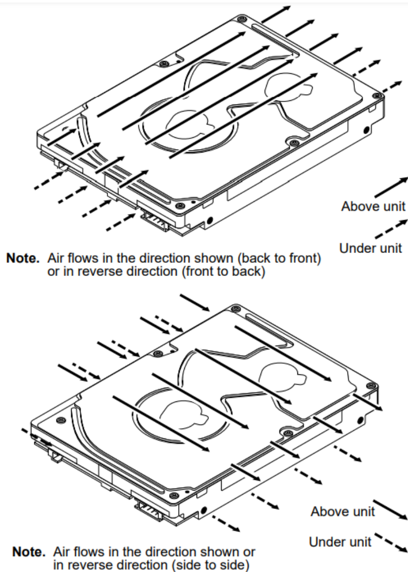
Figure 7. Air flow
