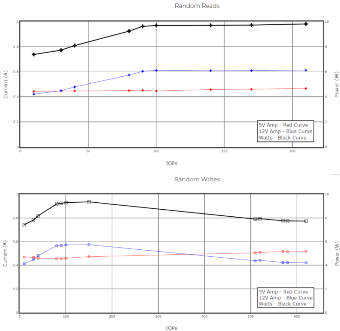
Figure 2. 24TB models (12Gb) DC current and power vs. input/output operations per second.
