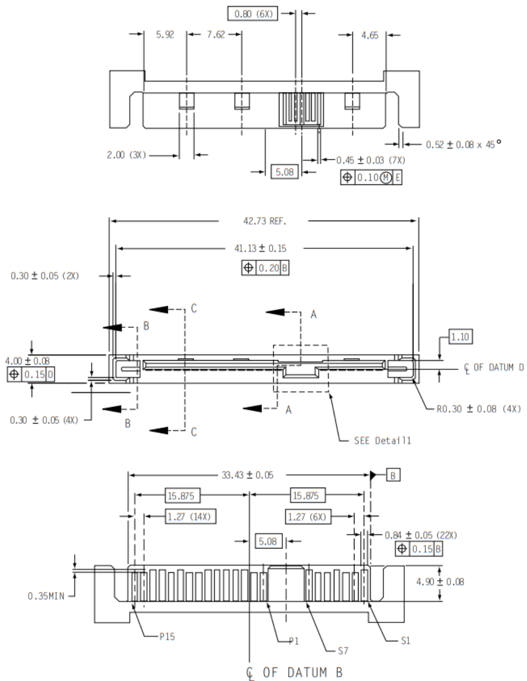
Figure 9. SAS device plug dimensions
