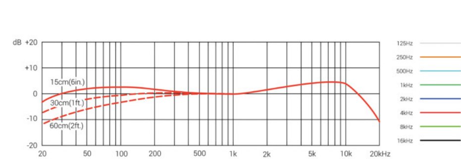
Frequency Response
