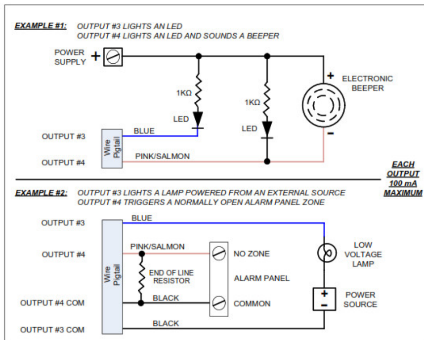
Fig. 5 Using Solid State Outputs
