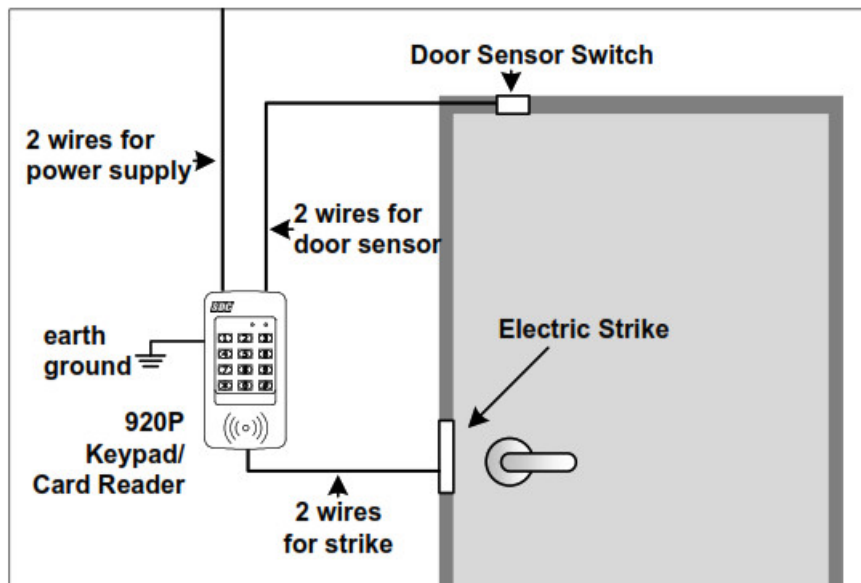
Fig. 3 Basic Door Installation
