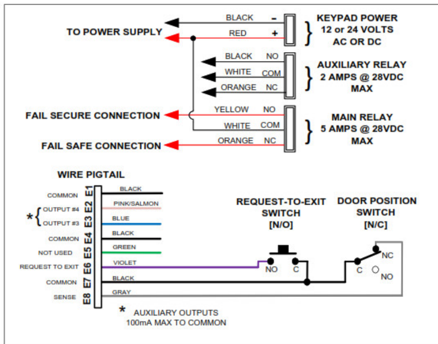
Fig. 4 Basic Door Installation Wiring
