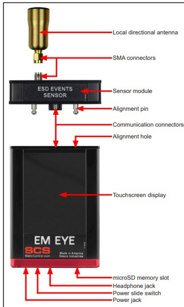
Figure 5. EM Eye features and components
