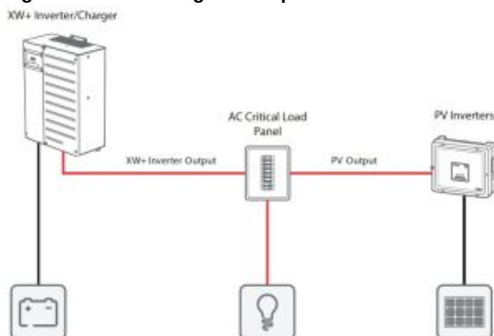
Figure 2 Grid Forming and Surplus Power
