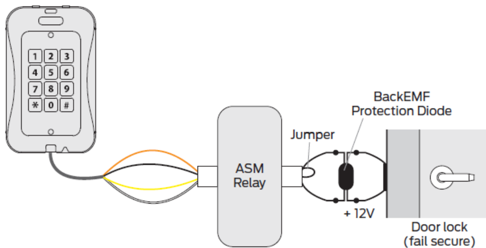
Figure 2.6: ASM with Reader Controller supplying PoE power
