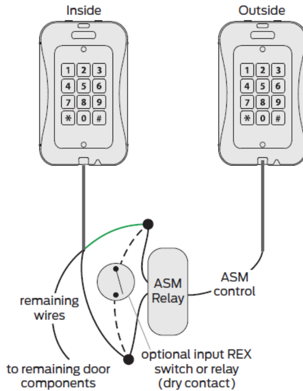
Figure 5.1: Two readers to one lock wiring
