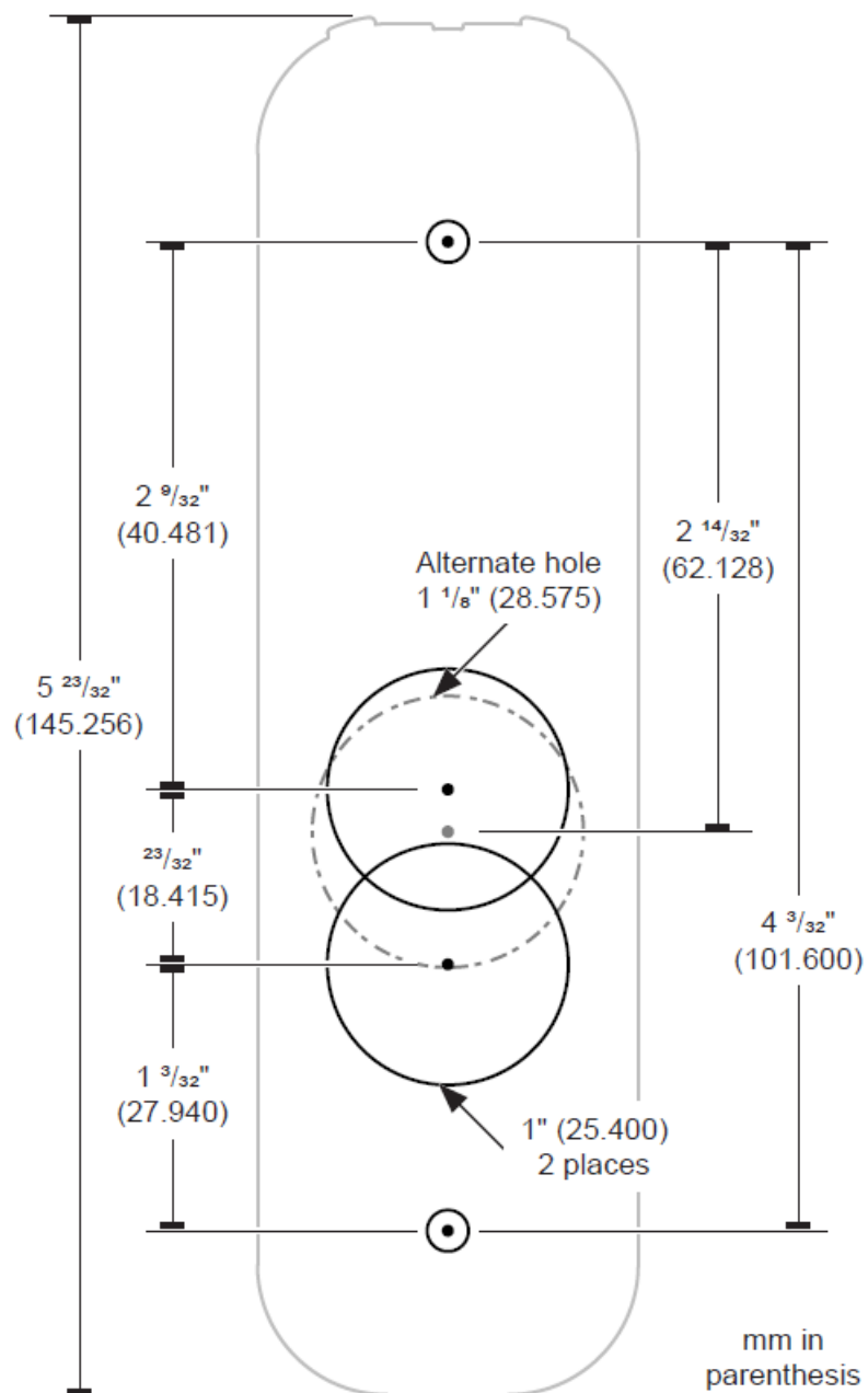
Figure 1.1: RC11 Mounting
