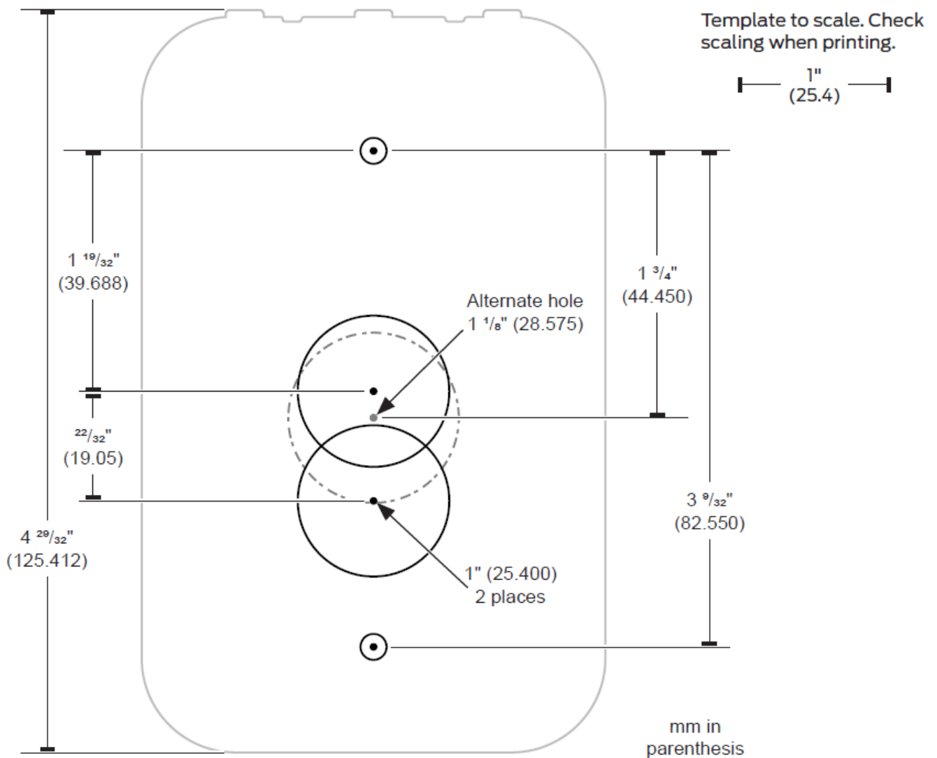
Figure 1.2: RC15/RCK15 Mounting
