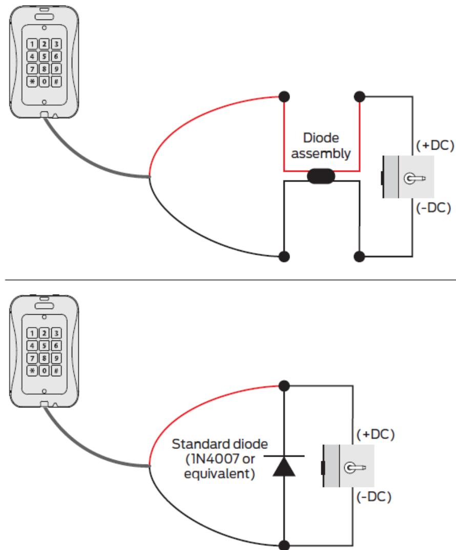
Figure 5.2: Inductive load control (two options shown)
