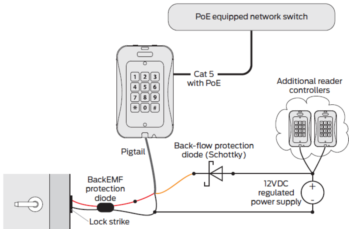
Figure 4.2: Dual power sources wiring
