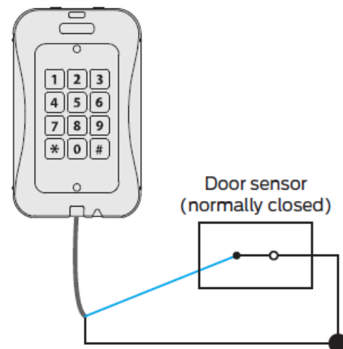
Figure 2.5: Door sensor wiring
