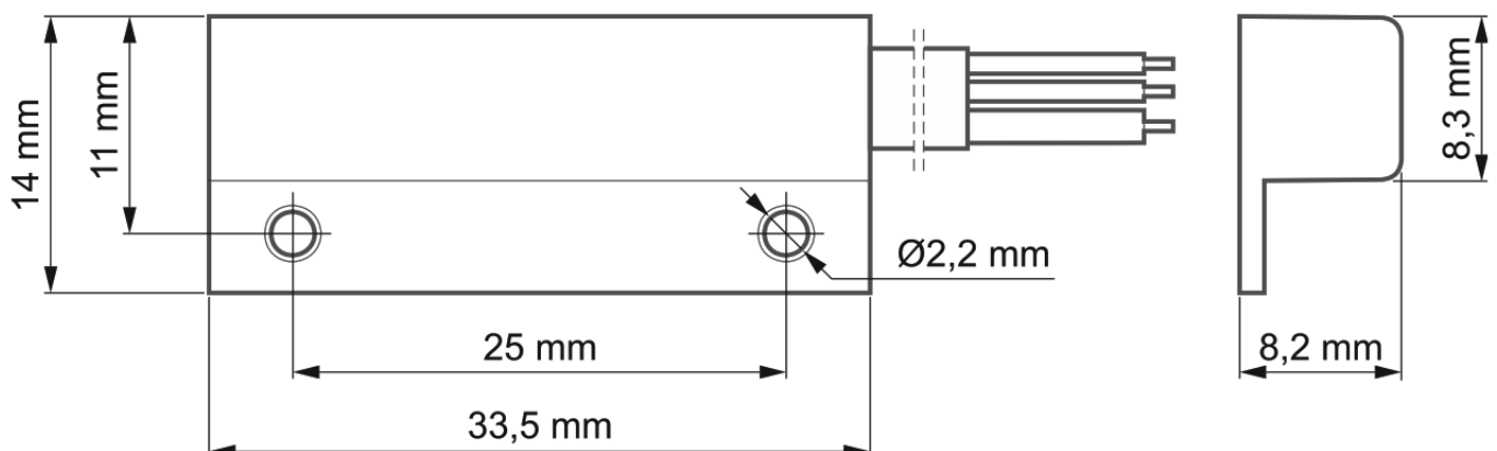
Fig. 3. Dimensions of DS-T1 temperature sensor enclosure.
