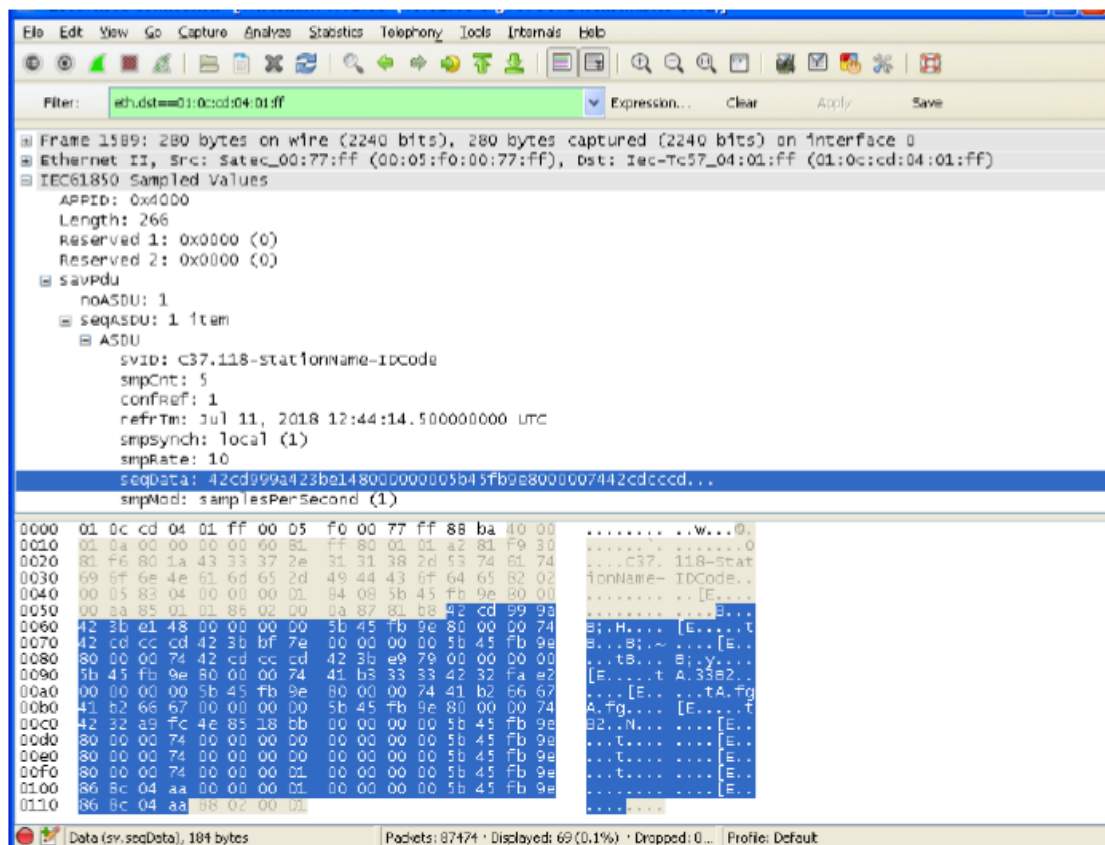
Figure 3-2 Captured synchrophasor multicast sampled values frame
