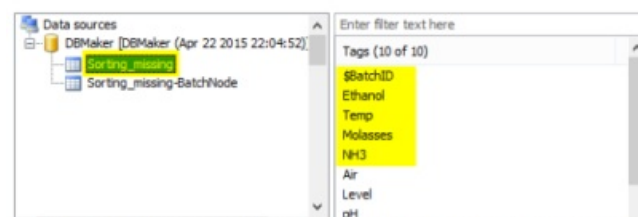
Figure 4: This is how the same node looks from SIMCA-online. You see the node name to the left, and the tags in that node listed to the right. The full tag path to the Ethanol tag in this screenshot is DBMaker.Sorting_missing.Ethanol .
