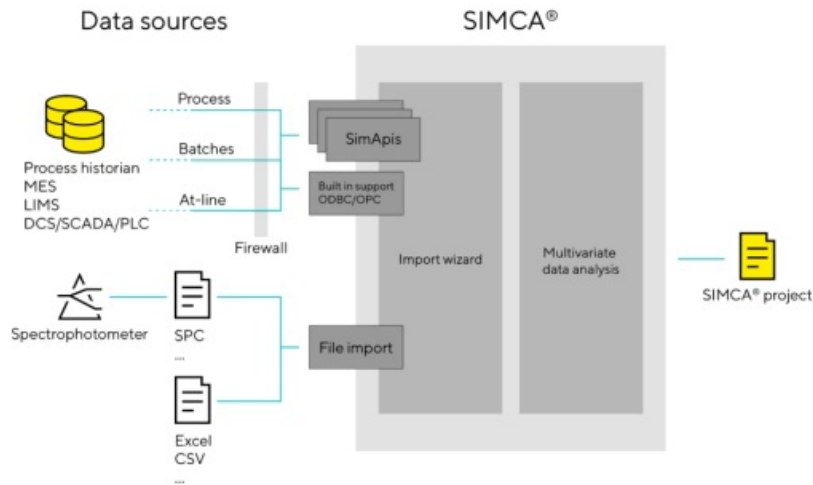
Figure 1. SIMCA used to obtain data from a data source through a SimApi.
