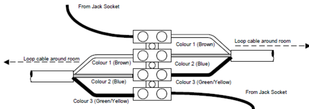
Junction Box Connections - 3-core Loop Cables
