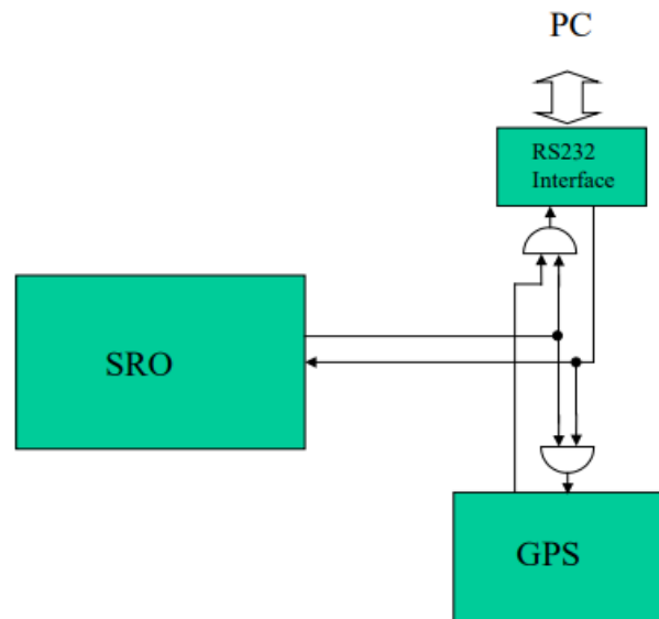
Figure 2: Communication Diagram (Switch S6 to the left)
