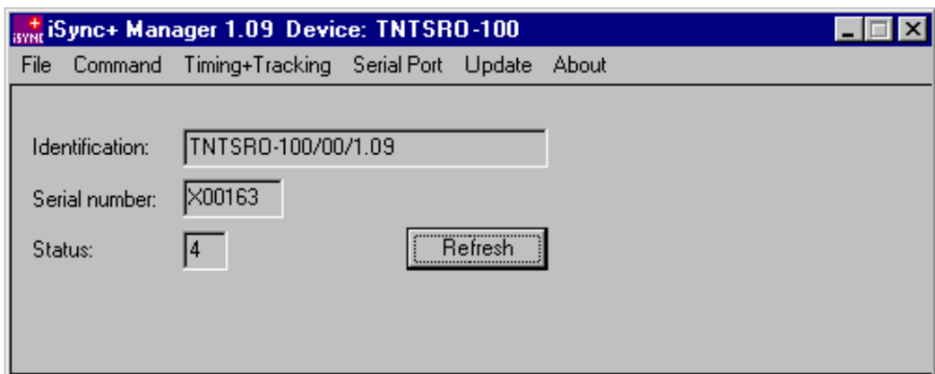
Figure 3: iSyncMgr.exe Program.
