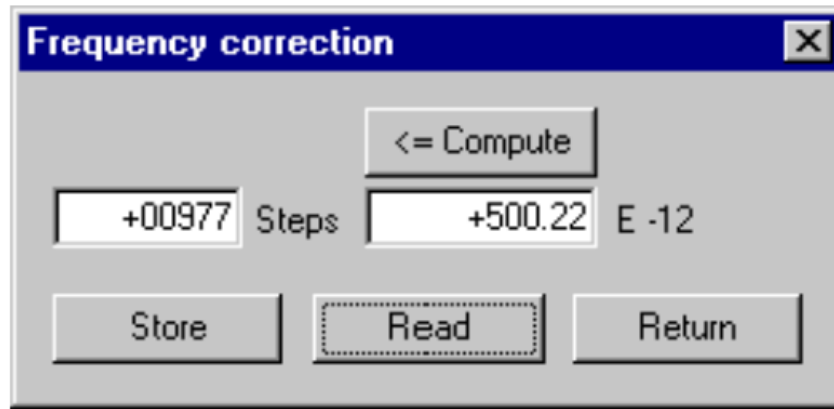
Figure 4: Frequency Correction in Free Run Mode.
