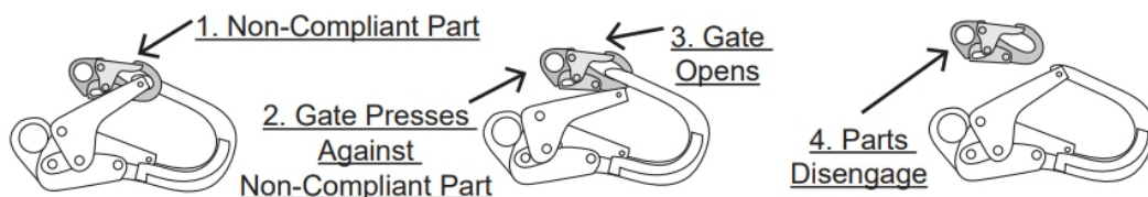
FIGURE 2: UNINTENTIONAL DISENGAGEMENT
