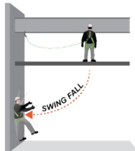
FIGURE 1: SWING FALL
