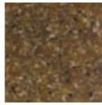
SANDSTONE
