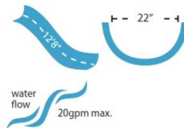
Flume Details
