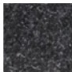
GRAY GRANITE
